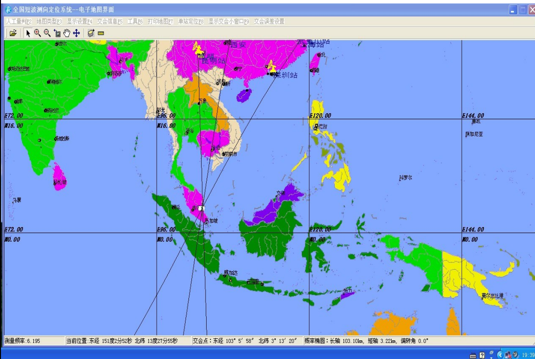
Figure 5 - Triangulation on 6 195 kHz
