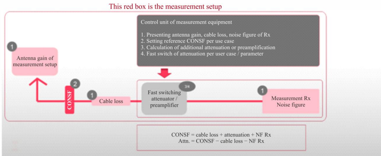
FIGURE 17 Implementation of calculated COSNF into the measurement setup
