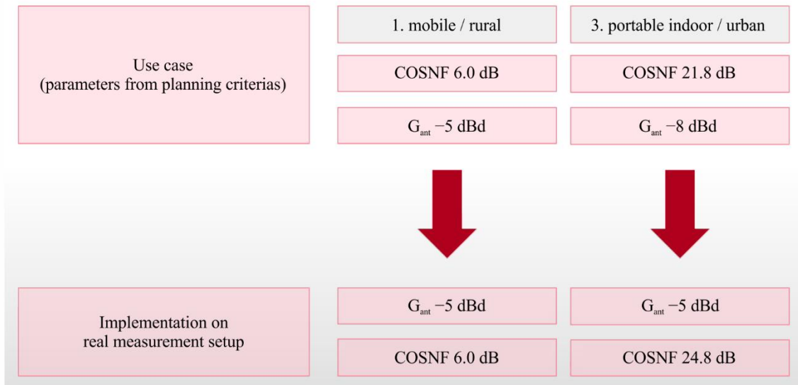
FIGURE 16 Implementation of COSNF
