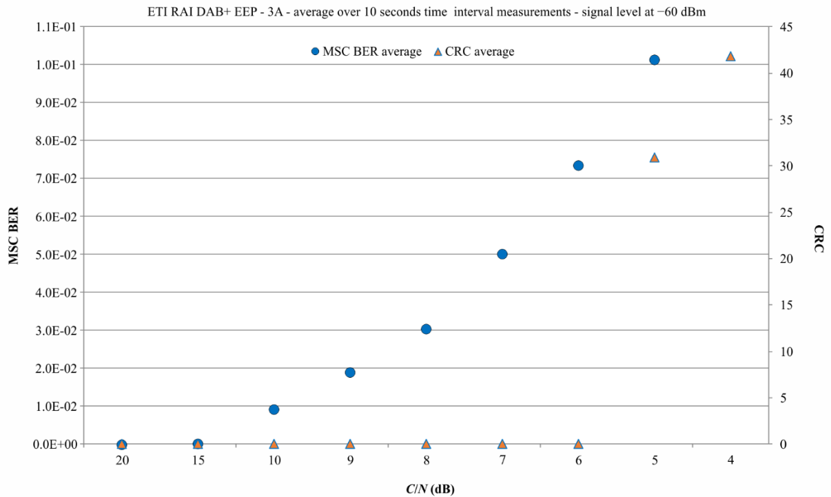
FIGURE 13 MSC BER and CRC averages with respect C/N
