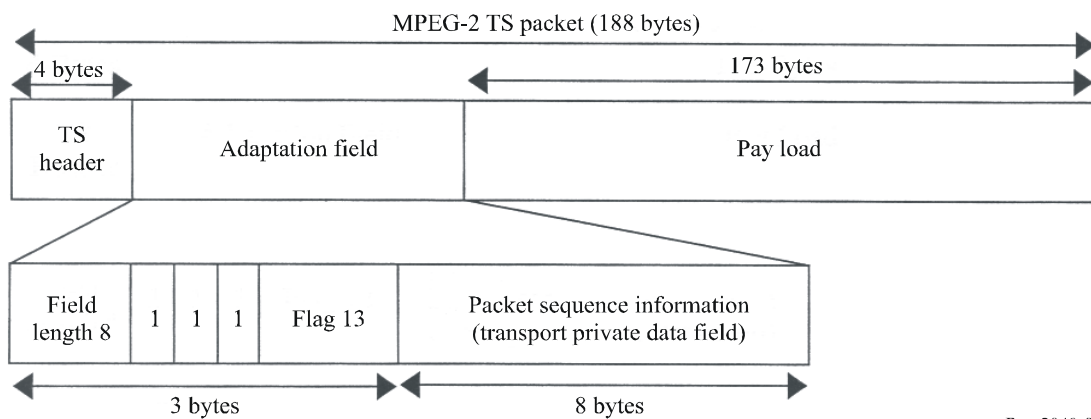
FIGURE 7 Proposed modification to add packet ID using 8 bytes in a private data field
