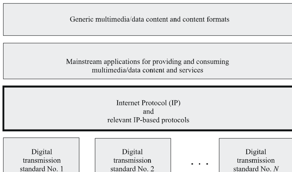
FIGURE 8 Internet Protocol and related protocols provide a common platform for multimedia and data broadcasting
