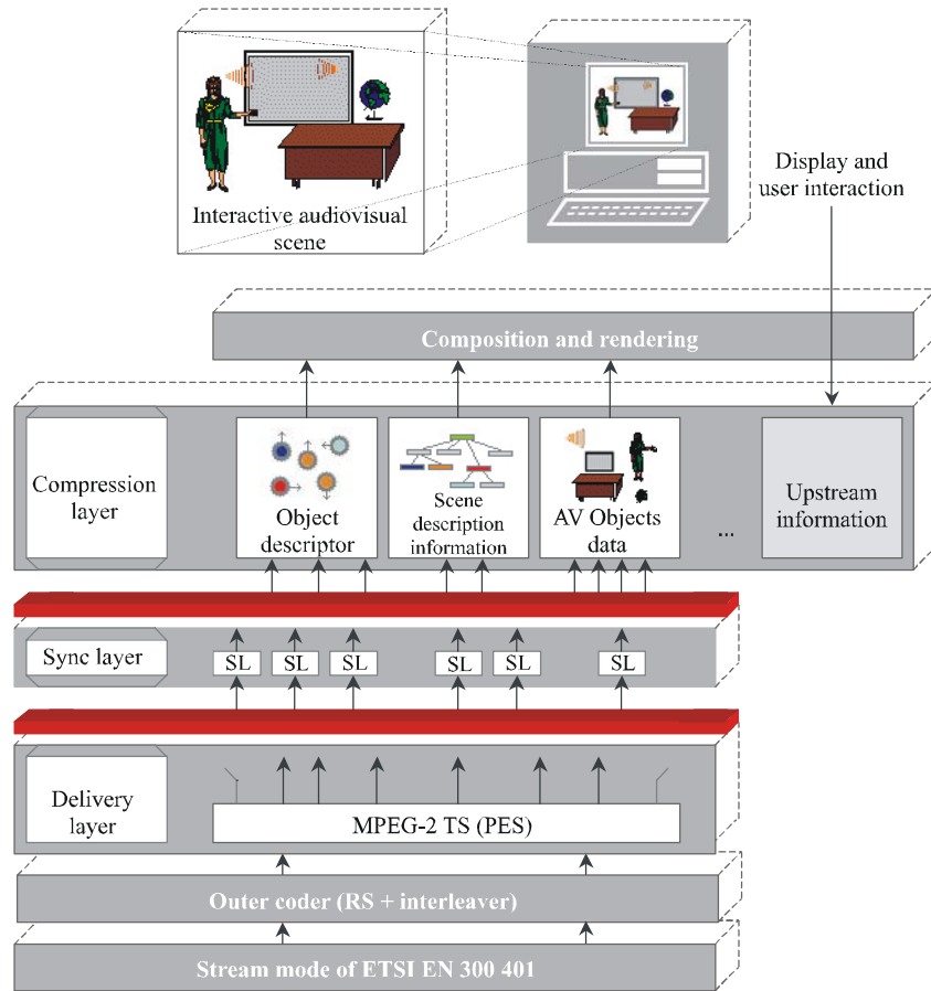
FIGURE 9 Conceptual architecture for the video services
