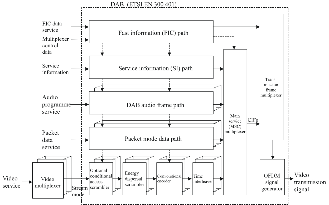
Conceptual transmission architecture for the video services
