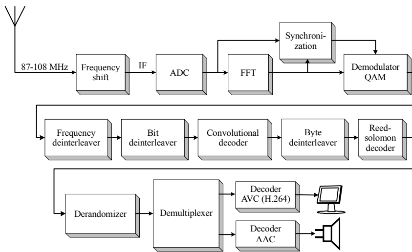
FIGURE 52 The receiver functional block diagram
