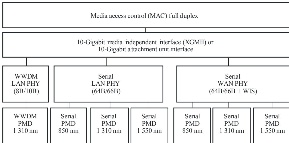
FIGURE 17 The architectural components of the 802.3ae standard
