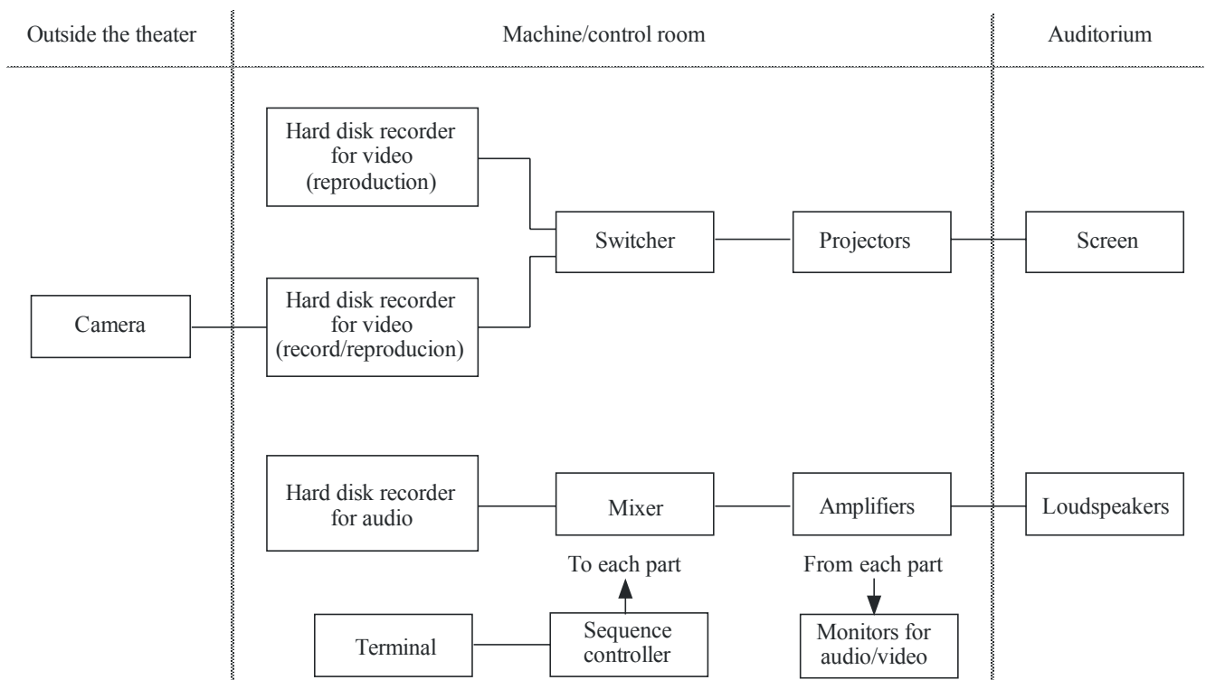
FIGURE 45 Schematic diagram
