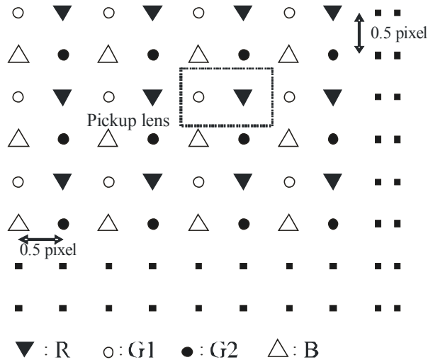
FIGURE 2 Relative positioning of pixels (Sampling position)
