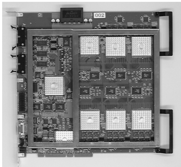
FIGURE 27 JPEG2000 decoder board
