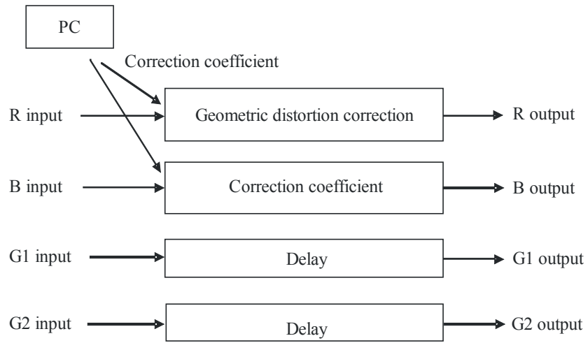
FIGURE 16 Configuration of convergence adjustment device
