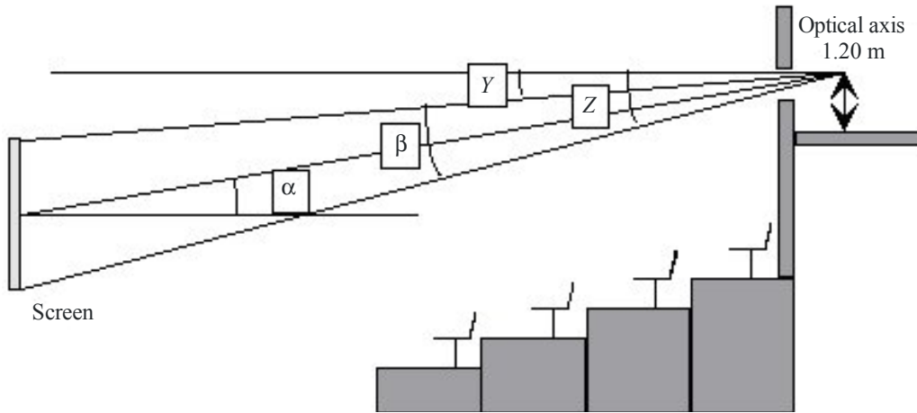
FIGURE 40 Image geometric distortion (vertical)
