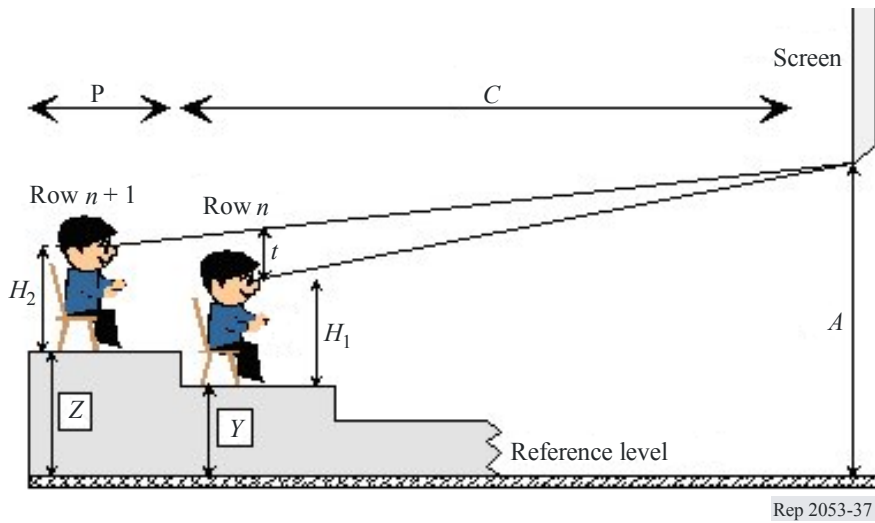
FIGURE 37 Head clearance
