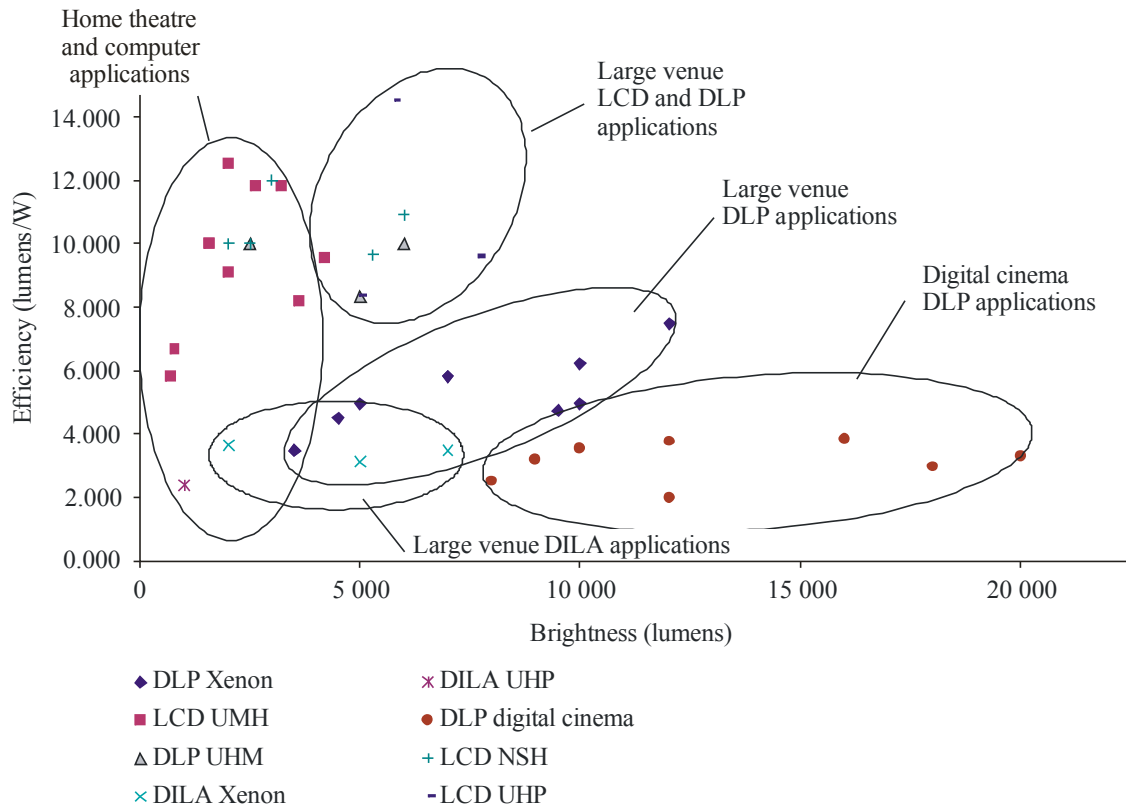
FIGURE 10 Plot of the projector efficiency to brightness Efficiency of projection technologies
