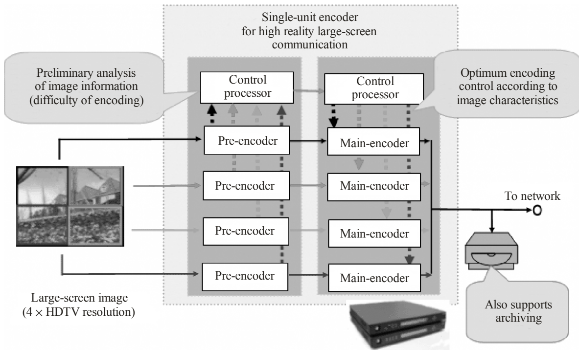
FIGURE 28 Spatially parallel encoding architecture for LSDI
