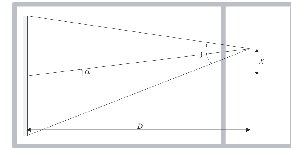
FIGURE 41 Image geometric distortion (horizontal)
