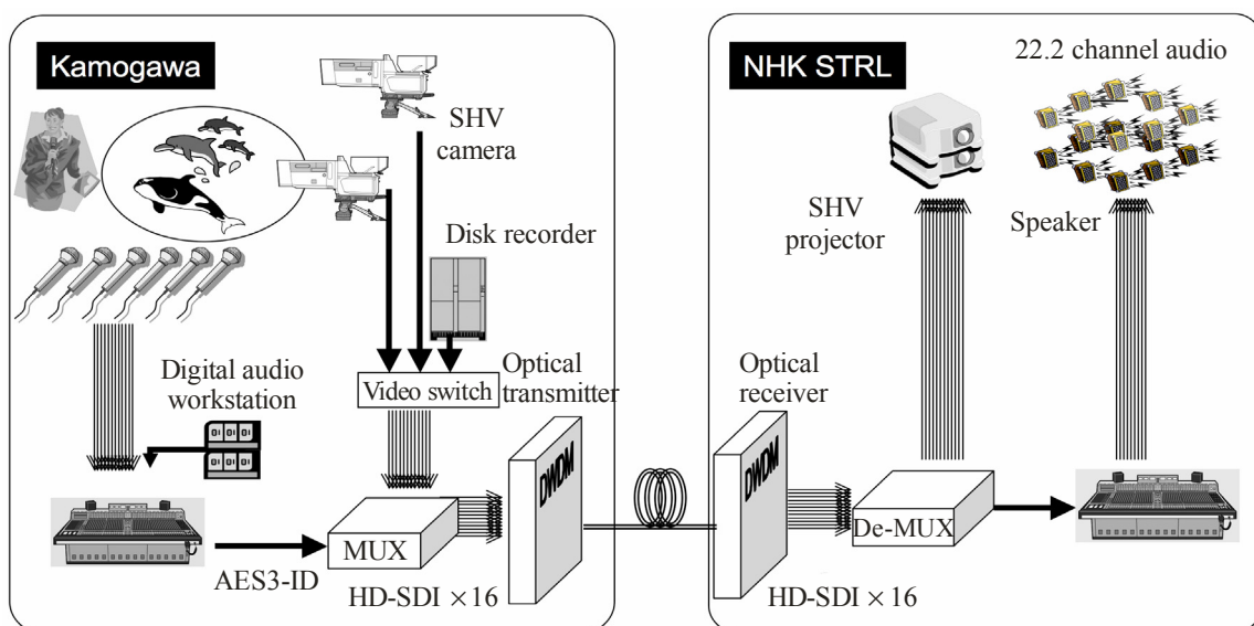
FIGURE 24 Schematic diagram of demonstration
