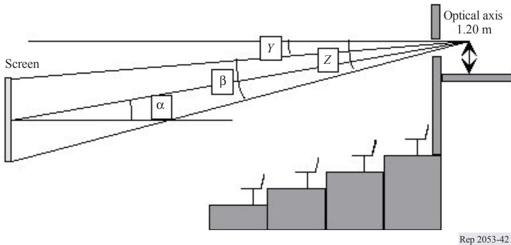
FIGURE 42 Clearance under projection beam
