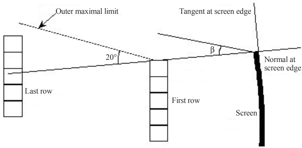
FIGURE 35 Side vision angle, curved screen
