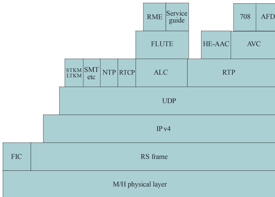
FIGURE 21 ATSC-M/H broadcast protocol stack
