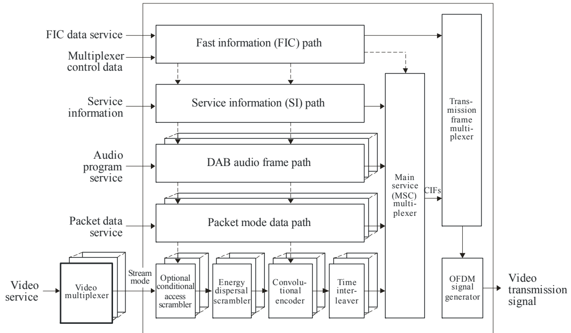
Conceptual transmission architecture for the video services DAB (ETSI EN 300 401)
