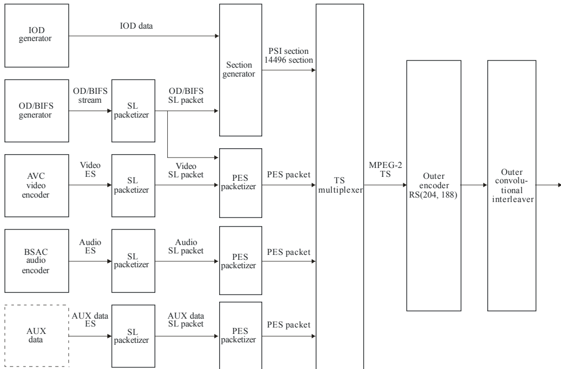
Architecture of the video multiplexer
