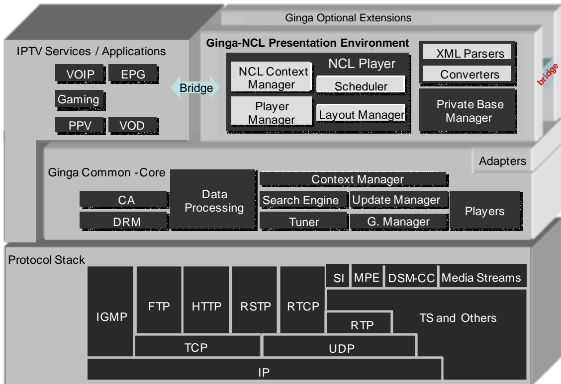
FIGURE 4.3 Ginga architecture
