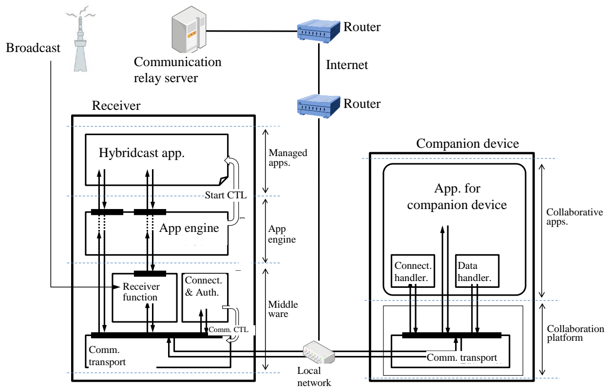
FIGURE 2.5 Entities and their relationship for companion device collaboration
