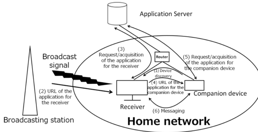
FIGURE 2.25 System configuration example of connecting a receiver and a companion device
