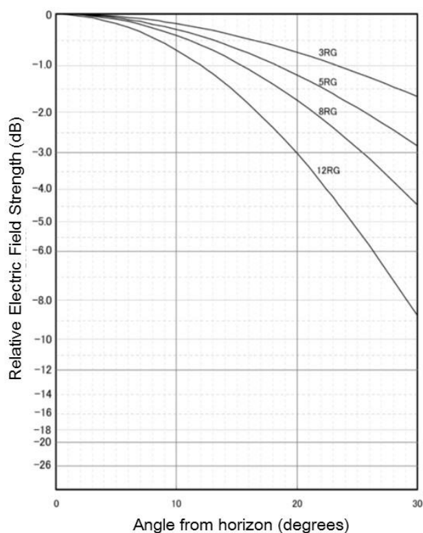
FIGURE 5 Vertical UHF radiation pattern for Repeater
