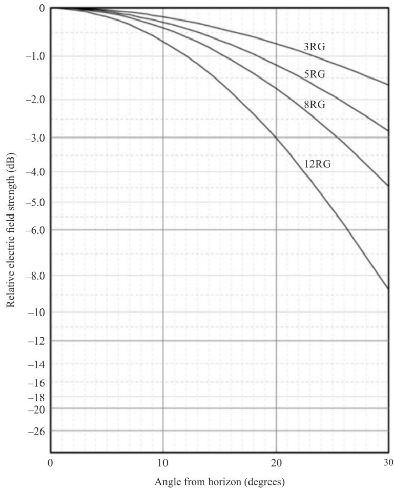
FIGURE 6 Vertical UHF radiation pattern for repeater
