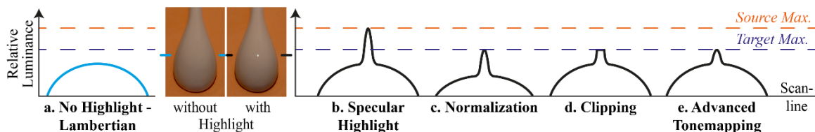
FIGURE 6 Effects of highlight rendering, clipping and (tonescale) compression
