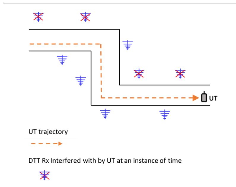
Impact of a moving interferer (user terminal) on DTTB reception
