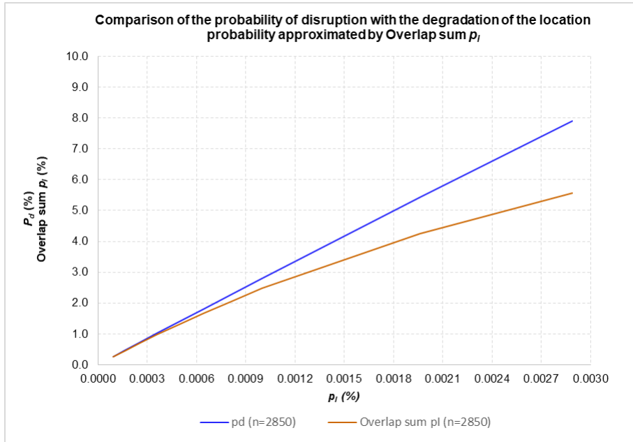
FIGURE 7 Relation between the probability of disruption and the degradation of the reception location probability n = 2\ 850
