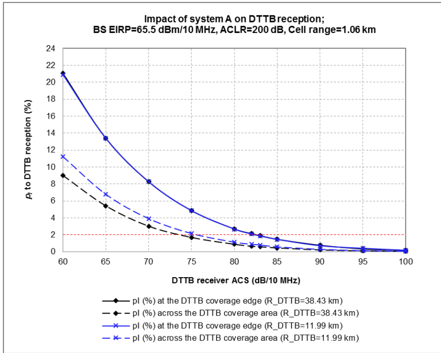
Figure 8 shows the variation of the p_I to DTTB reception as a function of the DTTB receiver ACS, for two different DTTB coverage radii: 38.43 km and 11.99 km for high and medium power DTTB transmitters respectively.
