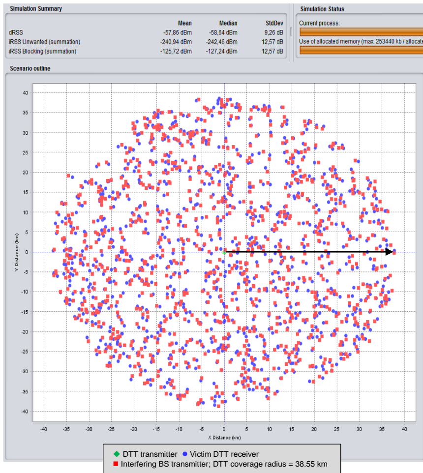
FIGURE 2 Several consecutive events generated by Monte Carlo simulation
