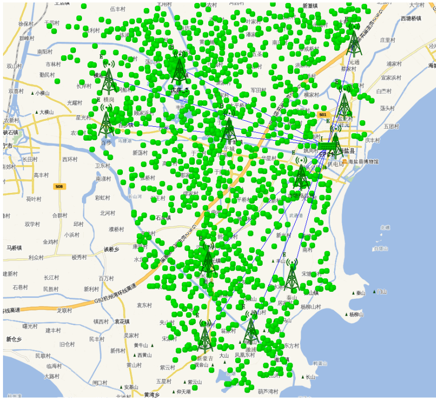
FIGURE 21 Deployment diagram of SWIN-based private power wireless network in Haiyan
