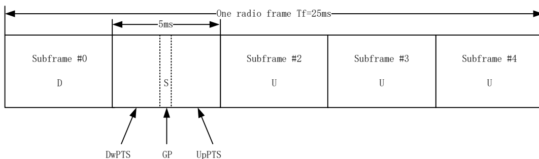
FIGURE 19 SWIN frame structure
