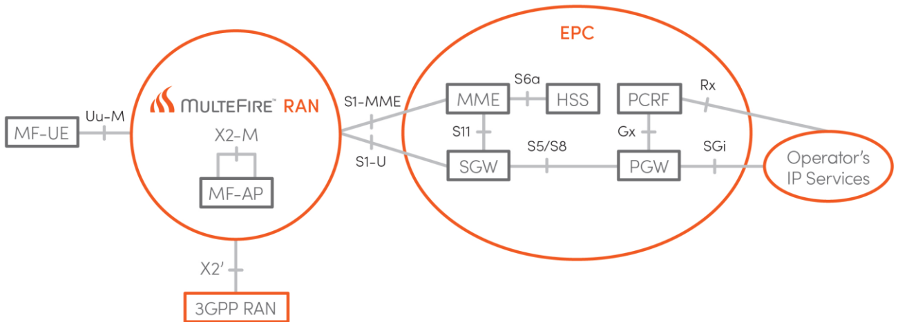
FIGURE 23 Architecture model for MulteFire PLMN Access Mode
