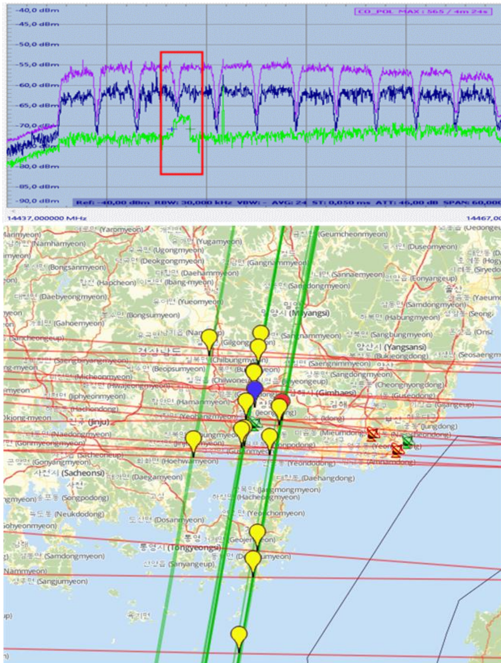
FIGURE 10 Searching interference source
