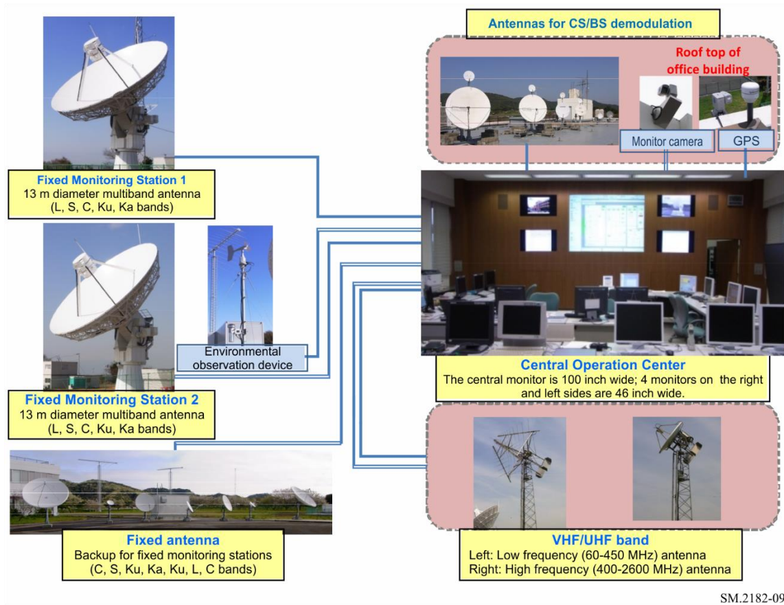
FIGURE 11 Configuration of the space radio monitoring facilities
