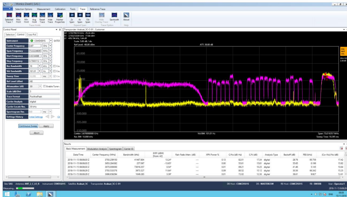
FIGURE 31 Reception of two different polarizations (Note: Main Pol = Yellow Trace, Cross Pol = Purple Trace)
