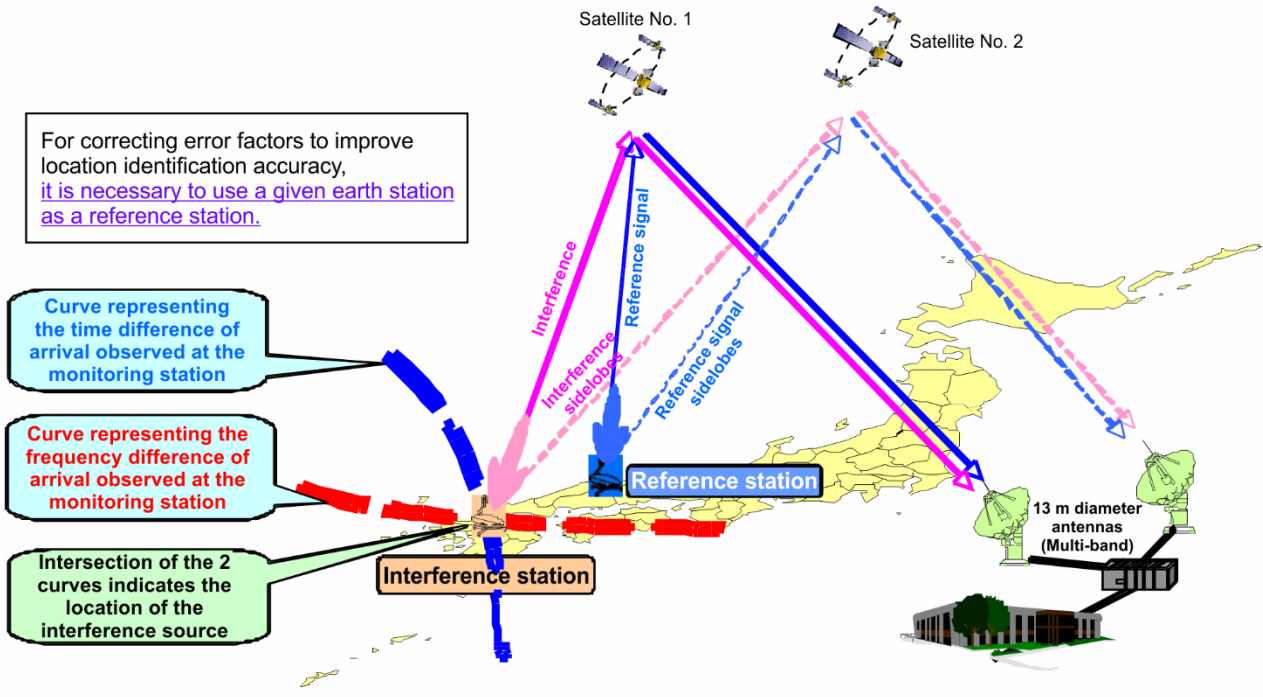
FIGURE 18 Mechanism of the uplink interference source identification system
