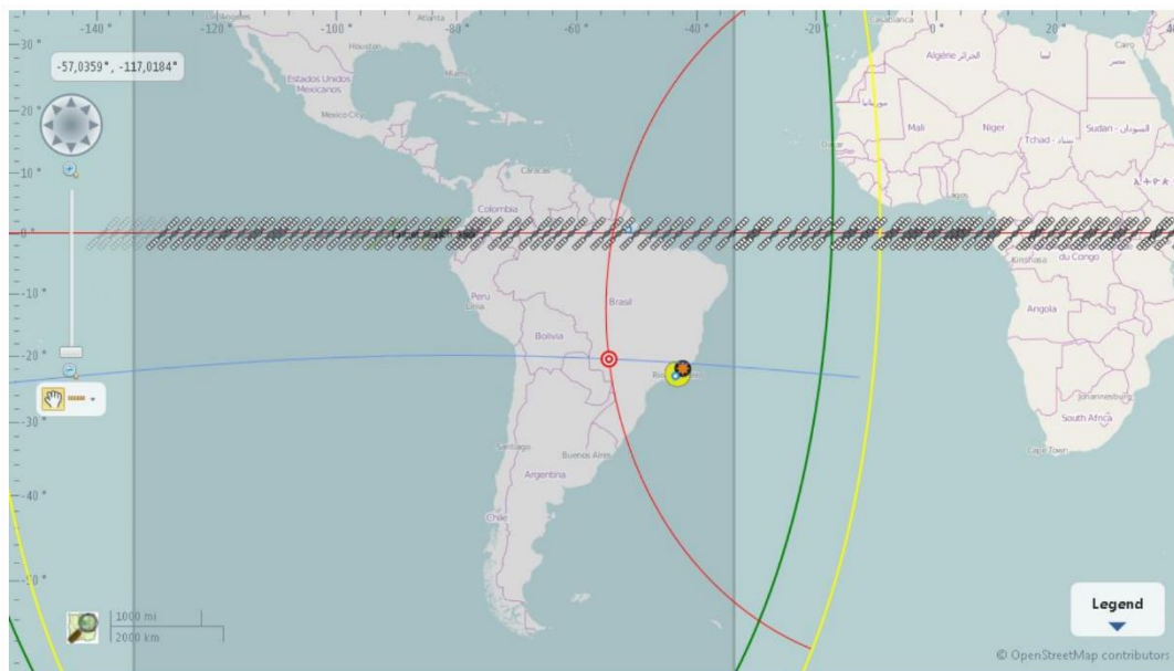
FIGURE 25 Geolocation output results (TDOA and FDOA lines and target indication)
