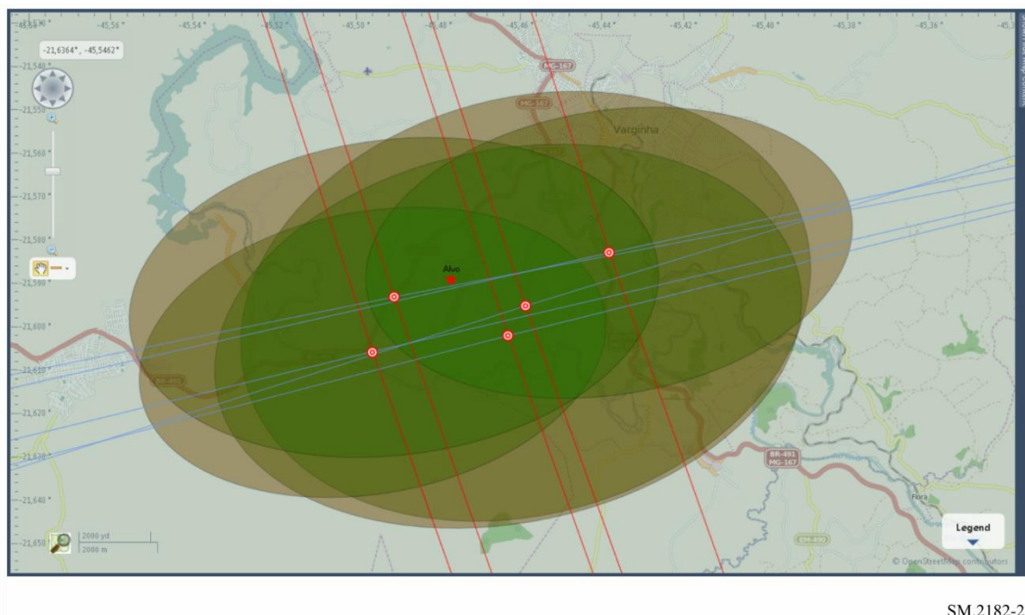
FIGURE 27 Geolocation output results (Geolocation ellipsis repeated five times and converging to same region)
