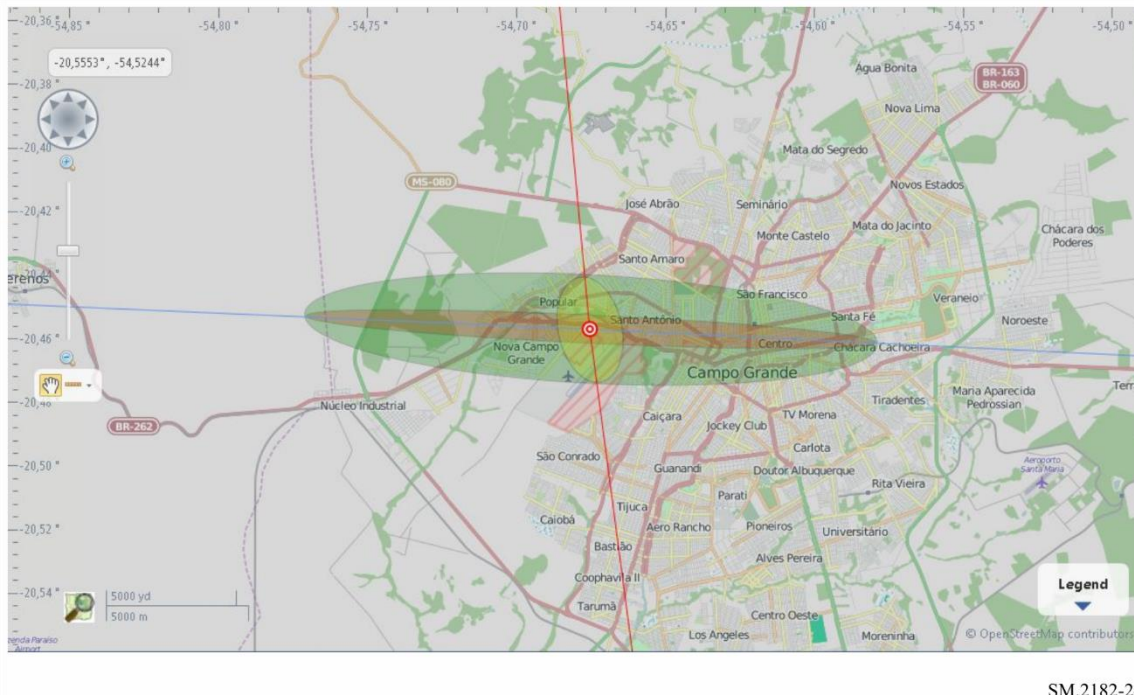
FIGURE 26 Geolocation output results (Geolocation ellipsis)
