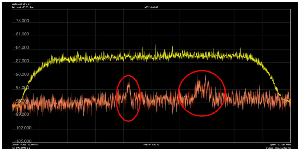
FIGURE 32 Carrier under carrier analysis
