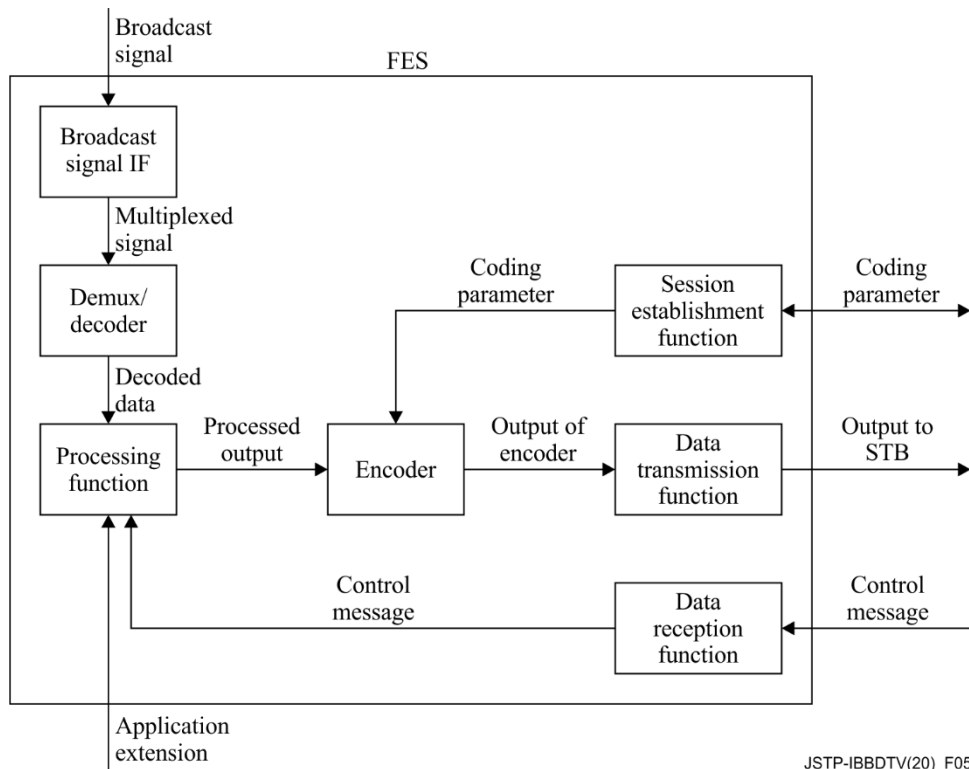
Figure 5 – Block diagram of processing server
