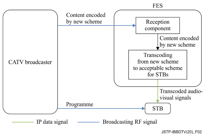
Figure 2 – Use case 1: Utilizing an advanced function
