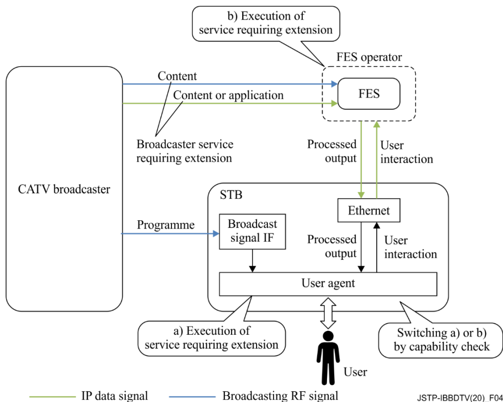
Figure 4 – Architecture overview of IBB digital TV application cooperating with the FES
