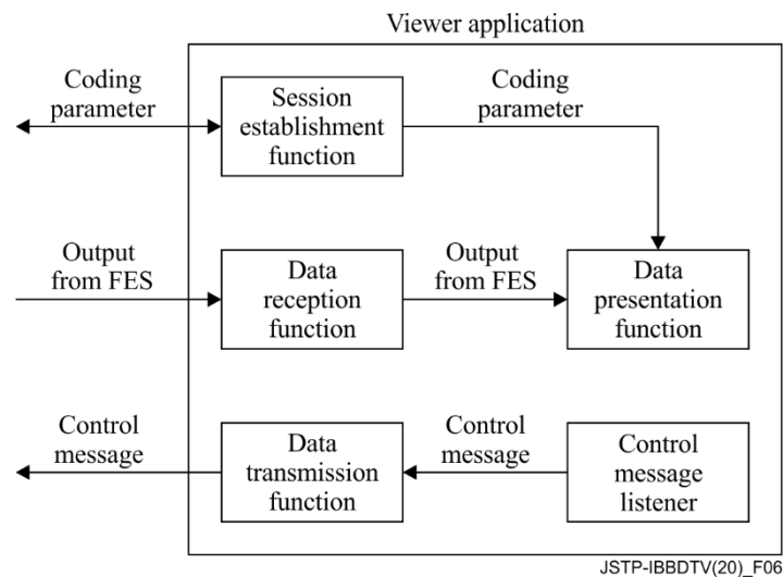
Figure 6 – Block diagram of viewer application
