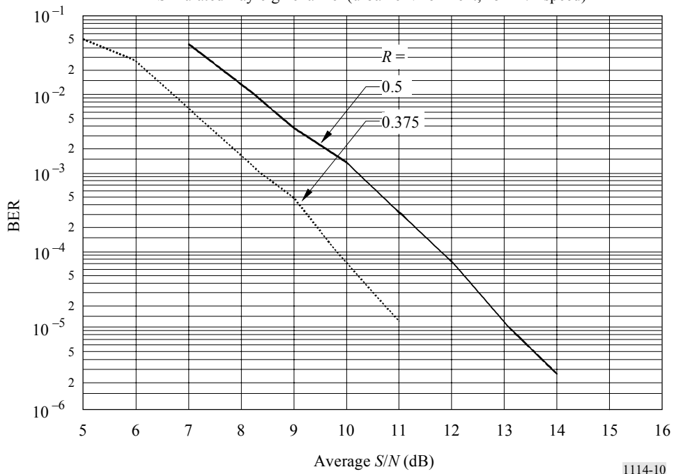
BER vs. S/N for System A (Transmission Mode I, 226 MHz)
