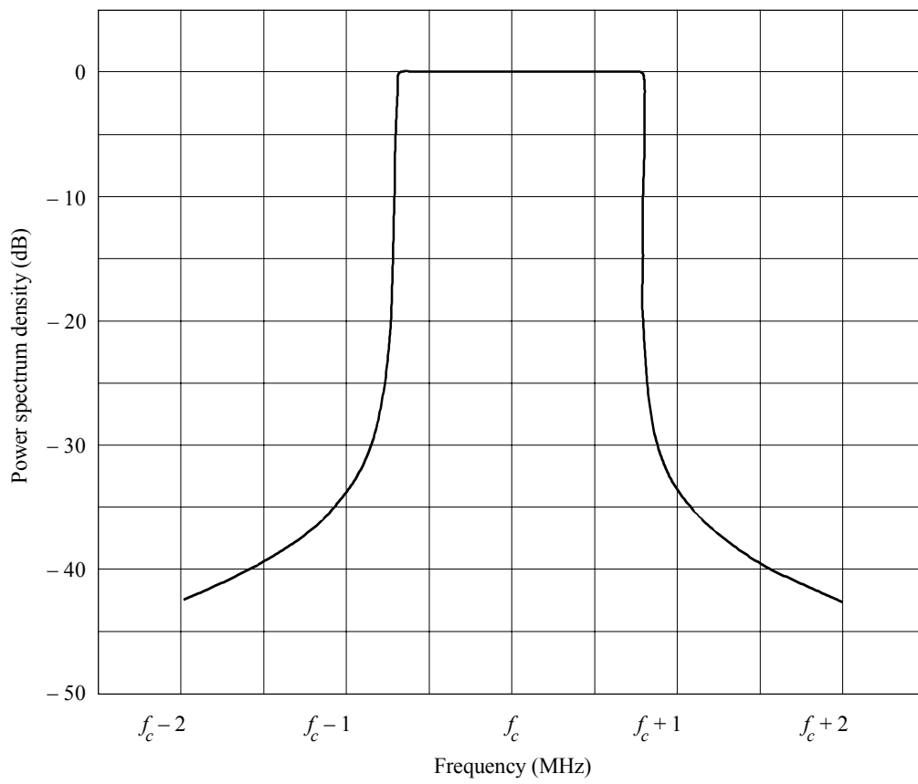
FIGURE 6 Theoretical transmission signal spectrum for transmission Mode II of System A
