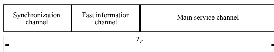
FIGURE 4 Multiplex frame structure
