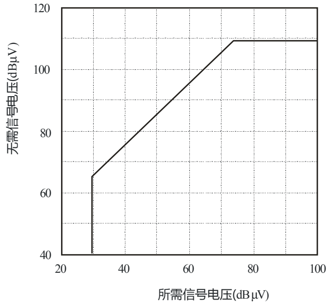
需要至干扰特性 (64-QAM-FEC 3/4)
