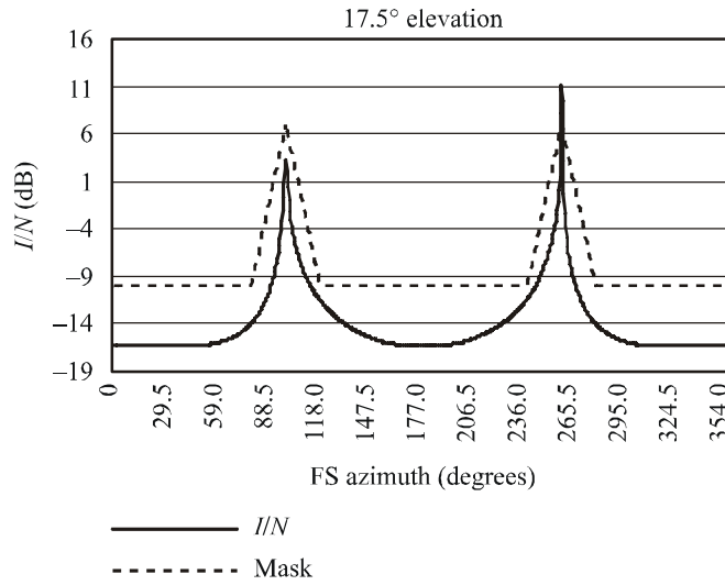
FIGURE 1 Description of I/N mask for GSO satellites in the 38 and 40 GHz bands
