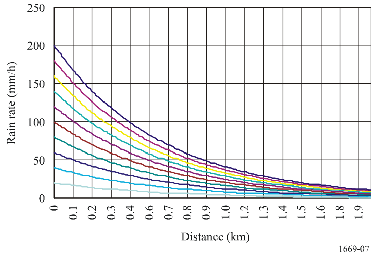
Rain rate from the centre of the rain cell
