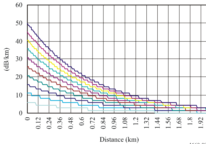
Specific attenuation from the centre of the rain cell
