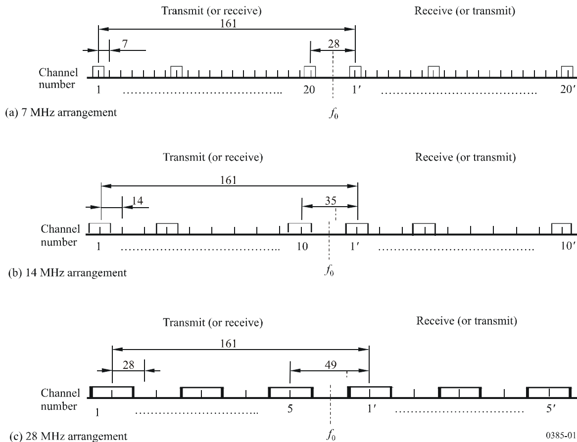
FIGURE 1 RF channel arrangement for international connection of FWSs operating in the 7 GHz band (All frequencies in MHz)
