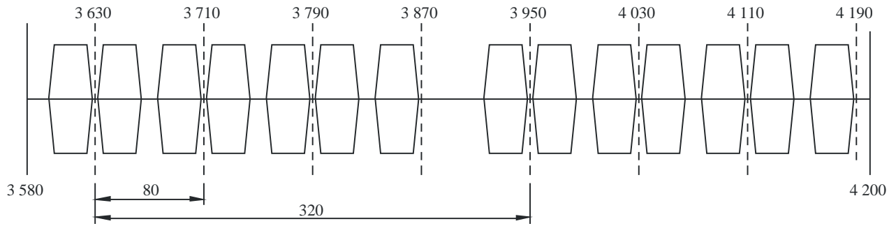
a) Channel arrangement in the band 3 580-4 200 MHz using a 2-carrier system transmitting (12 + 2) \times 155.52 Mbit/s (STM-1) in CCDP mode as available in Germany
