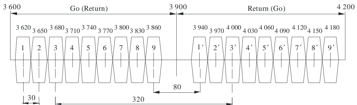
FIGURE 5 Radio-frequency channel arrangement for the 4 GHz band (All frequencies in MHz)
