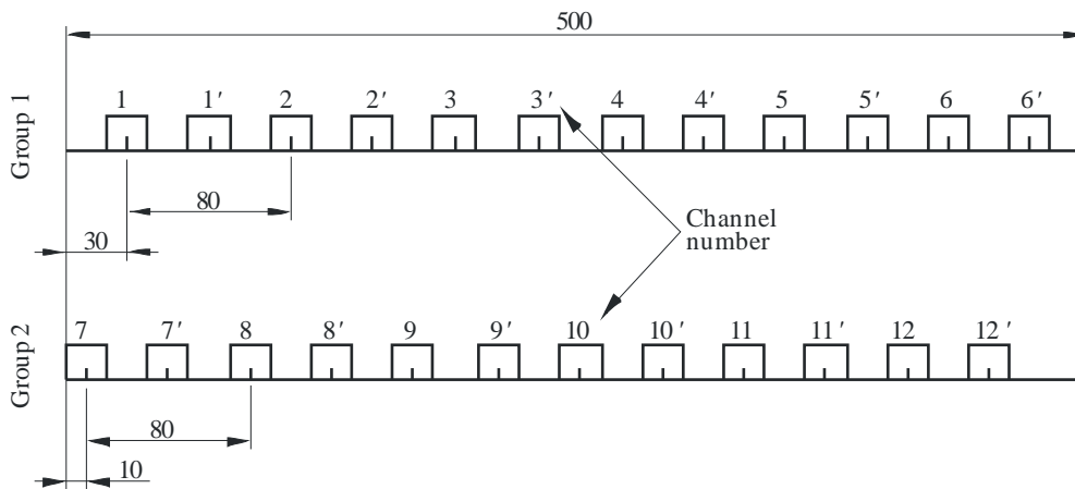
FIGURE 3 Radio-frequency channel arrangements for the 3.7-4.2 GHz band (All frequencies in MHz)
