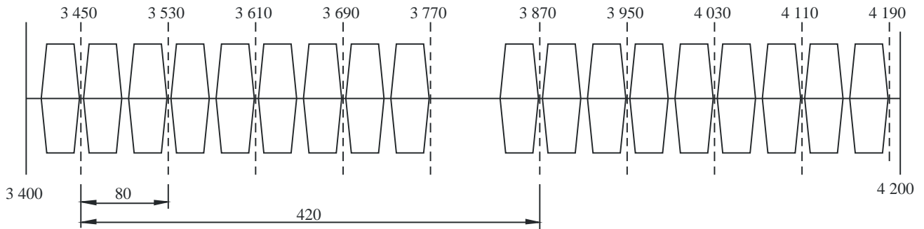
b) Possible channel arrangement in the band 3 400-4 200 MHz using a 2-carrier system transmitting (16 + 2) \times 155.52 Mbit/s (STM-1) in CCDP mode
