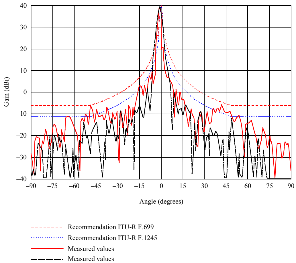
FIGURE 5 21 GHz lens horn P-P antenna of 50 cm diameter ( D/\lambda = 37 ; gain = 40 dBi)
