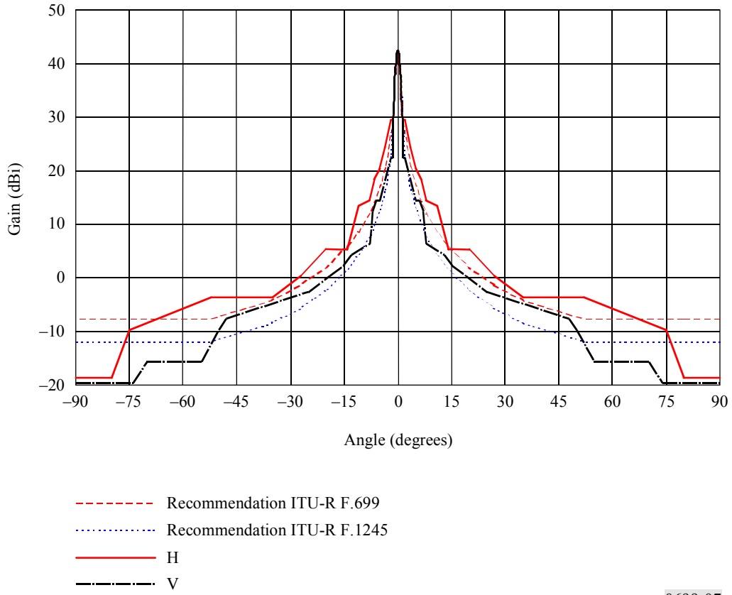
FIGURE 7 55 GHz P-P antenna of 0.3 m diameter ( D/\lambda = 57 ; gain = 42.4 dBi) (H: horizontal polarization, V: vertical polarization)
