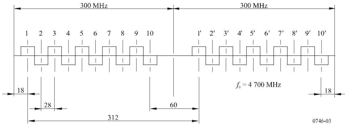
FIGURE 3 Radio-frequency channel arrangement for the band 4 400-5 000 MHz with a 28 MHz channel spacing
