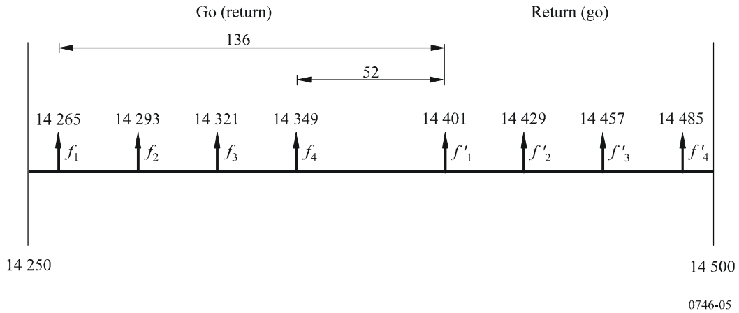
FIGURE 5 Radio-frequency channel arrangements for FWSs operating in the 14 GHz band with 28 MHz separation (All frequencies in MHz)
