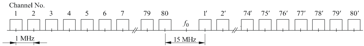
FIGURE 2 Radio-frequency channel arrangement for up to 300 telephone channel FWSs operating in the 2 300-2 500 MHz band
