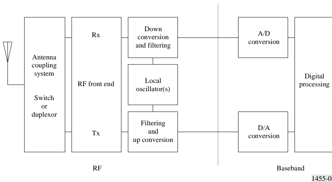
FIGURE 1 General block diagram of an IMT-2000 device
