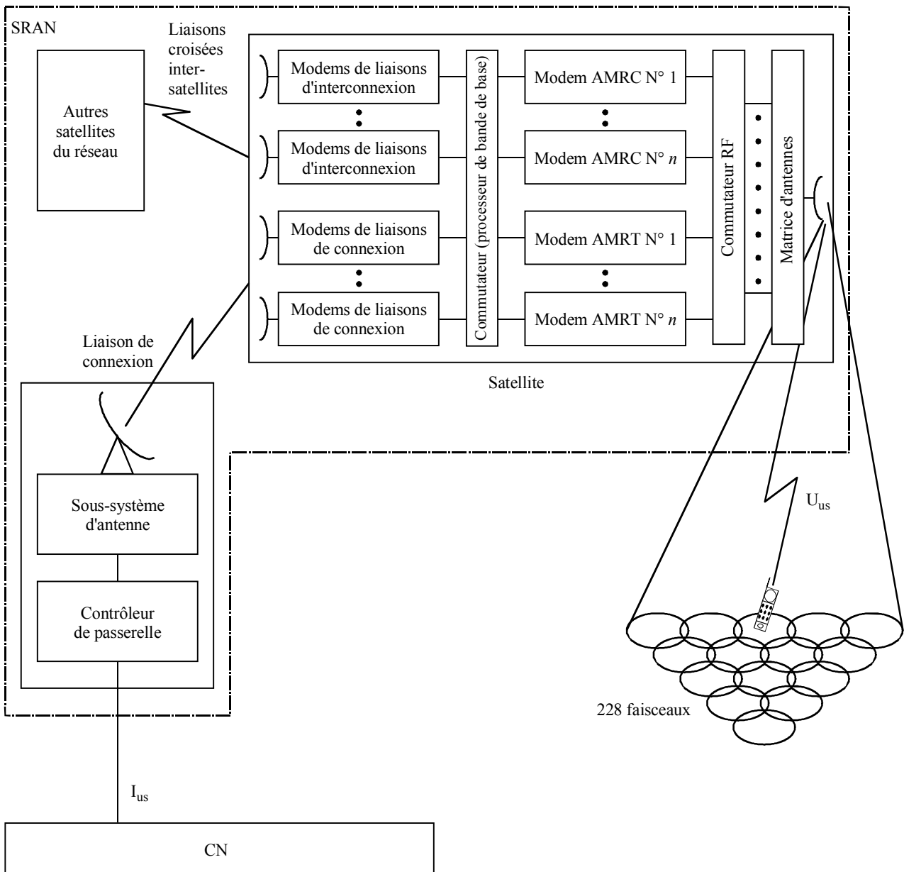
FIGURE 113 Architecture de Satcom2000
