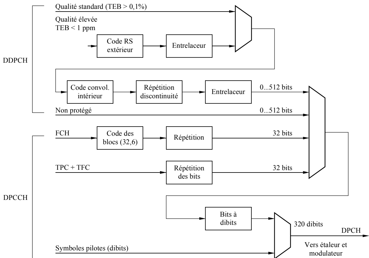
FIGURE 65 Codage et multiplexage
