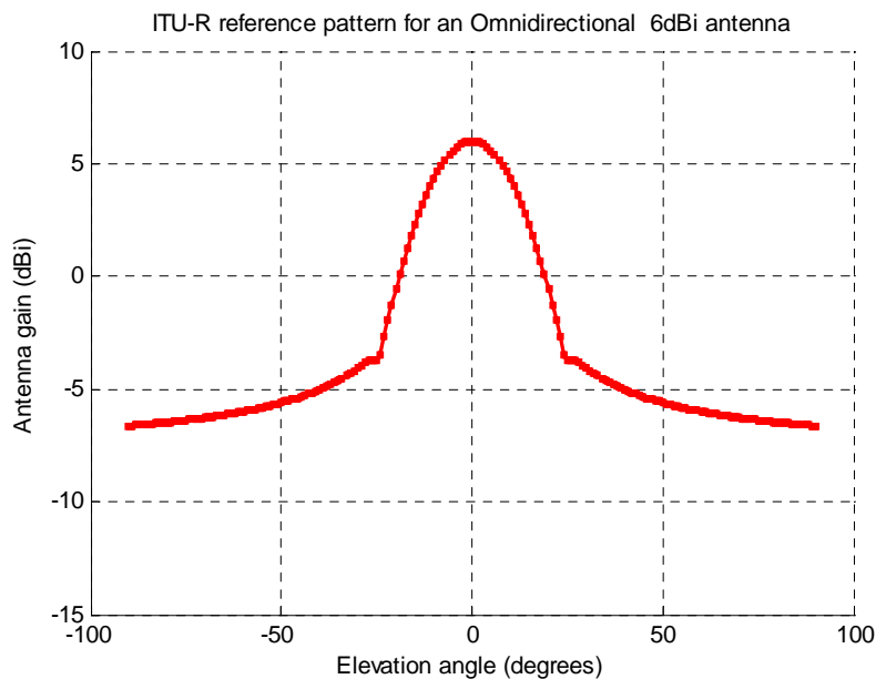
FIGURE 2 AM(R)S receiver antenna pattern
