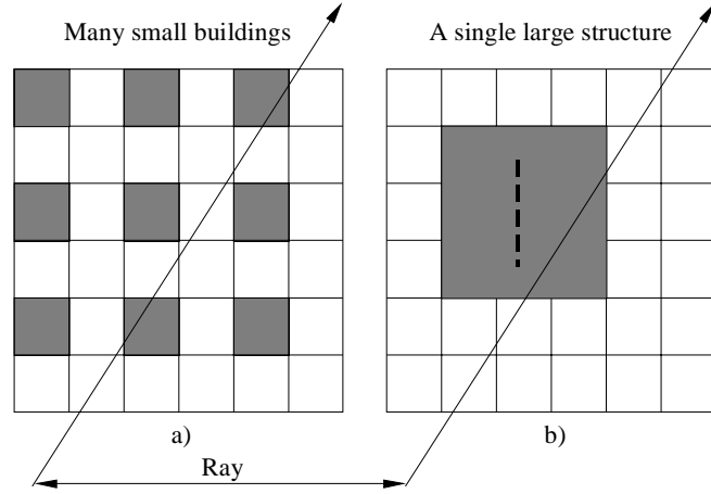
FIGURE 2 Two scenarios with the same area covered but different number of ray interactions
