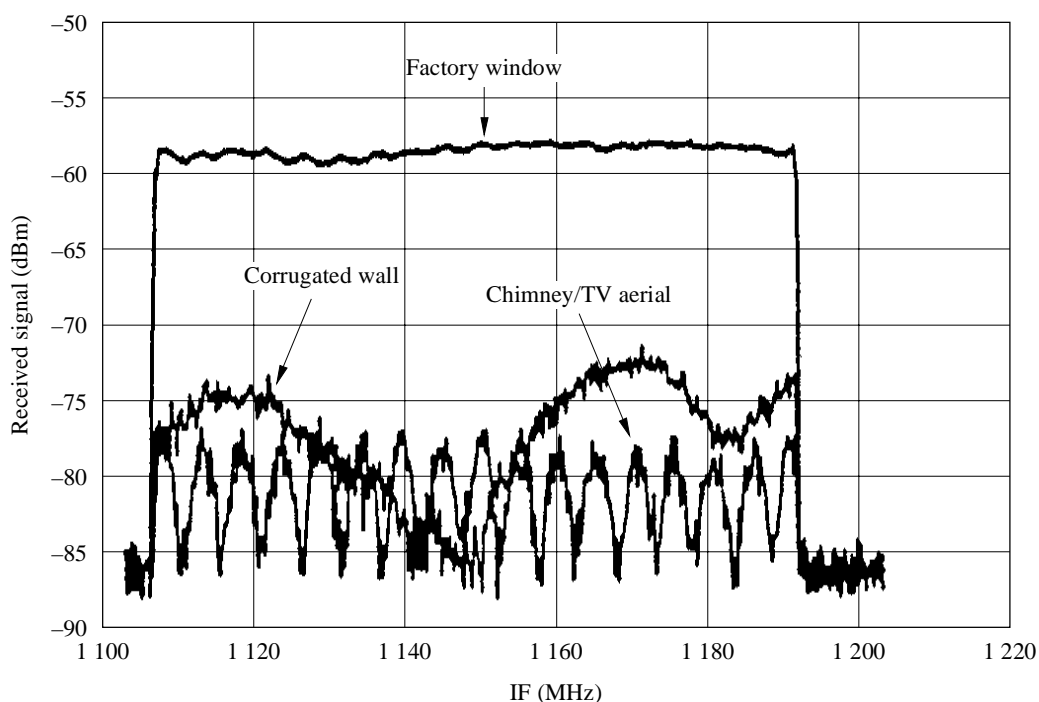
FIGURE 11 Frequency response for measured reflections at 3 different locations
