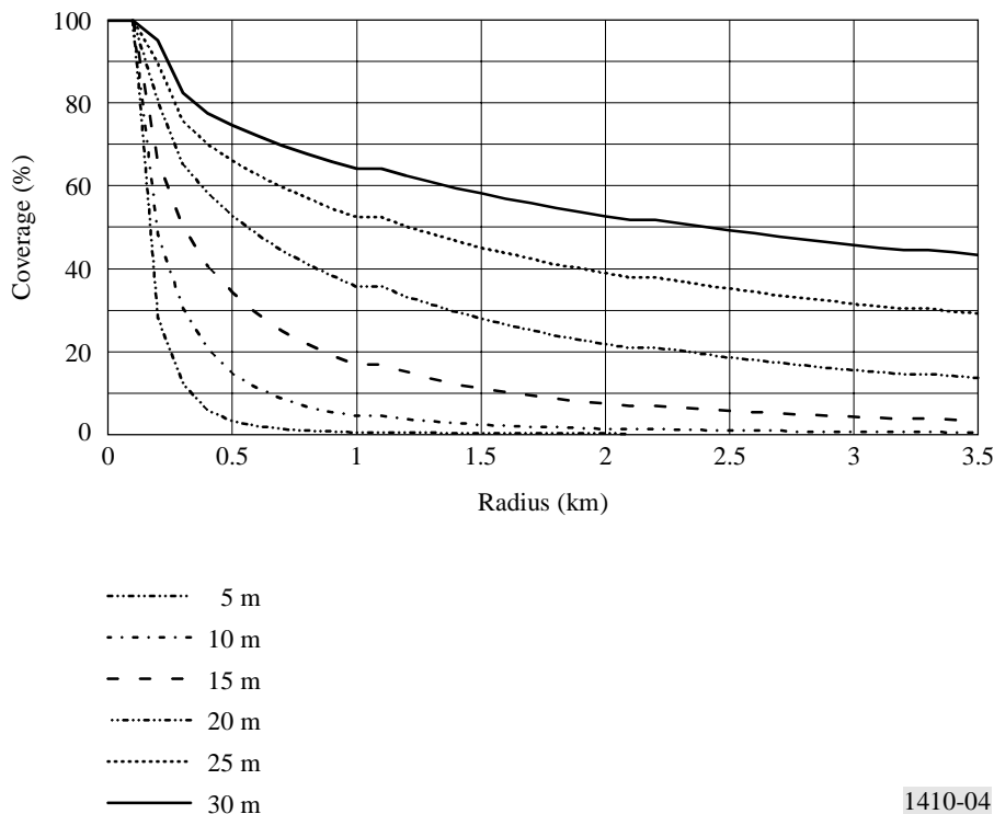
FIGURE 4 Modelled cumulative coverage for receiver at height of 7.5 m and transmitter at heights of 5, 10, 15, 20, 25 and 30 m
