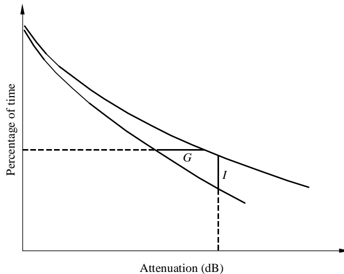
FIGURE 8 Example of attenuation statistics of path-angle diversity
