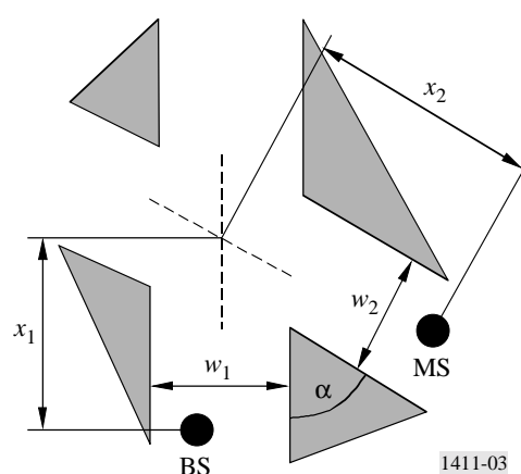
FIGURE 3 Definition of parameters for the NLoS2 case
