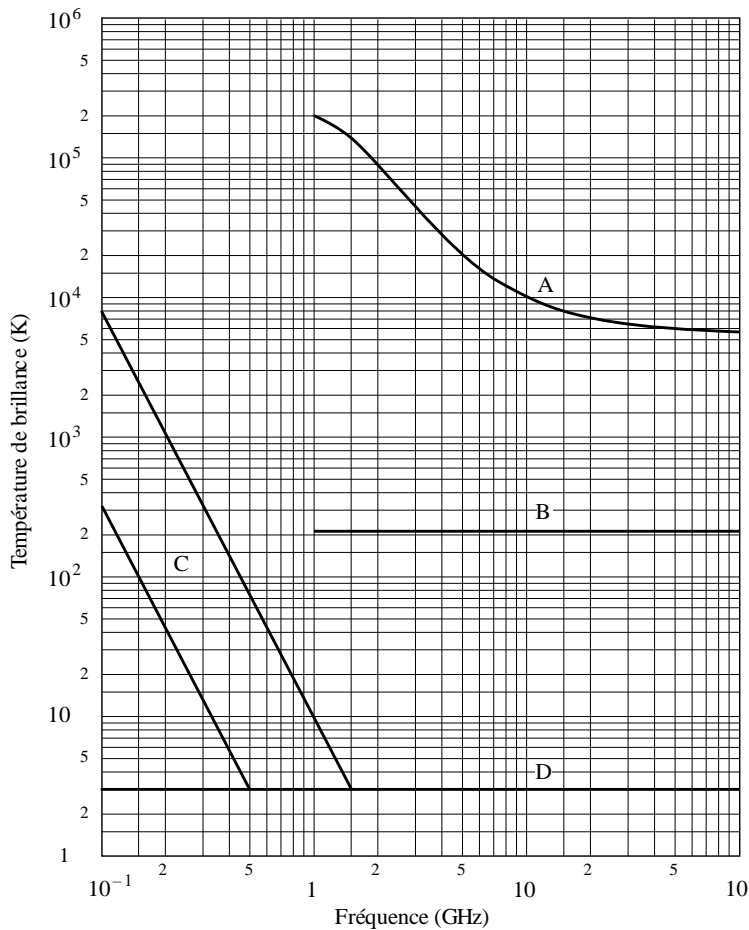
FIGURE 10 Sources de bruits extraterrestres
