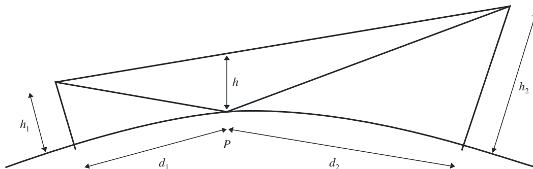
FIGURE 7 Path clearance
