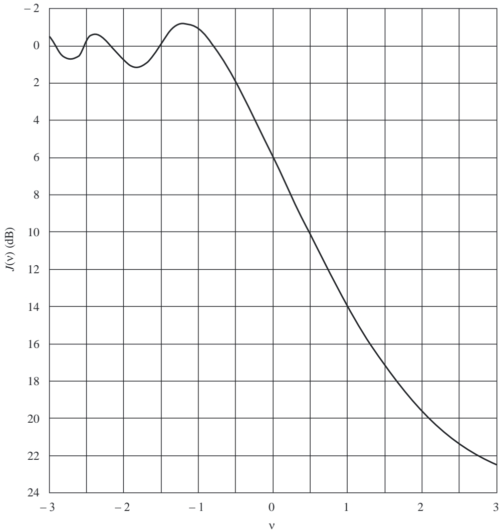
FIGURE 9 Knife-edge diffraction loss
