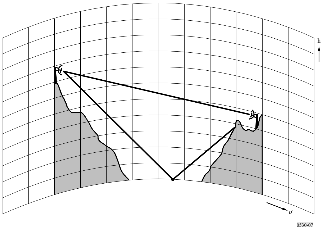
FIGURE 7 Example of shielding of antenna from specular reflection
