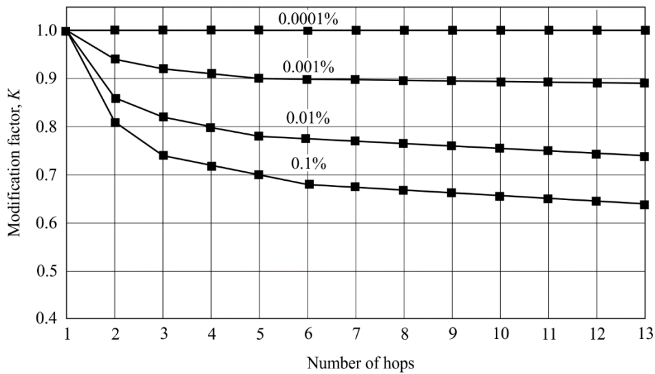
FIGURE 7 Modification factor for joint rain attenuation on a series of tandem hops of approximately 4.6 km each for several exceedance probability levels for each link (May 1975-March 1979)
