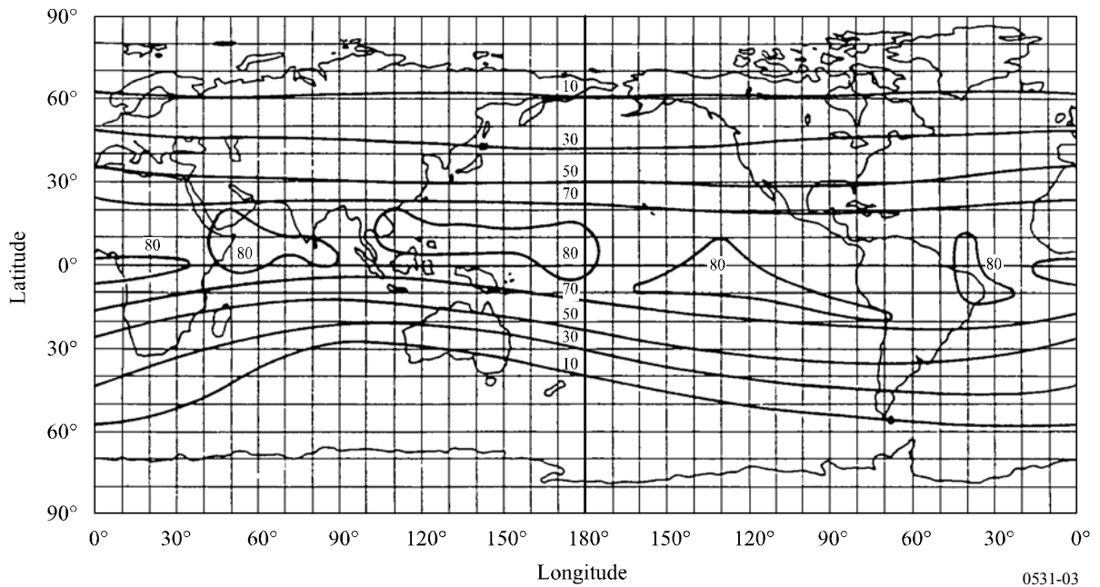
FIGURE 3 Contours of percentage of yearly average daytime hours when time delay at vertical incidence at 1.6 GHz exceeds 20 ns (sunspot number = 140)
