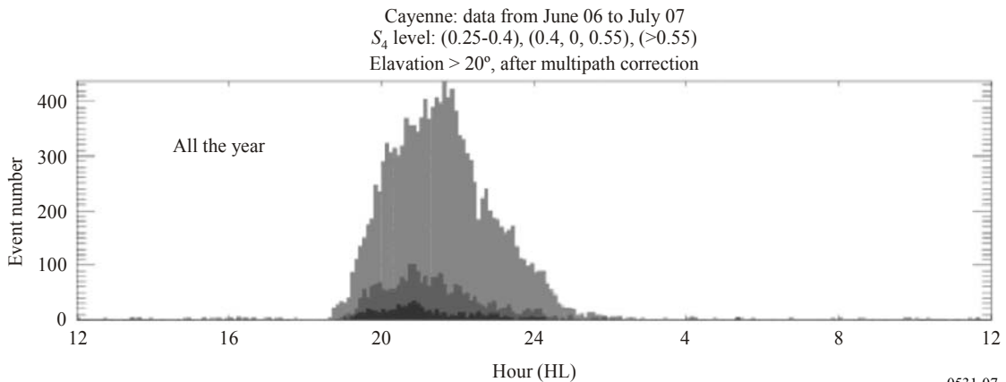
Distribution of one year scintillation events at Cayenne during June 06 to July 07; S_4 level weak (top); moderate (middle); strong (bottom) for elevation angles > 20^\circ
