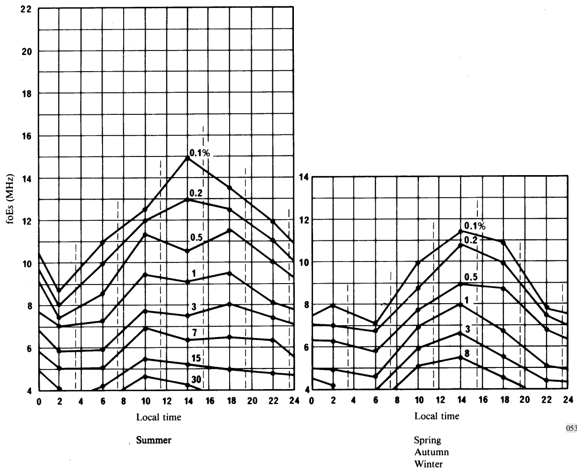
FIGURE 10 – Values of foEs equalled or exceeded for the percentage of time indicated as the parameter on the curve during time blocks shown separated by the dotted vertical lines of 4 hours for region D (South America)
