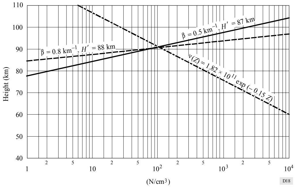
FIGURE 19 Ambient day and night constituent profiles
