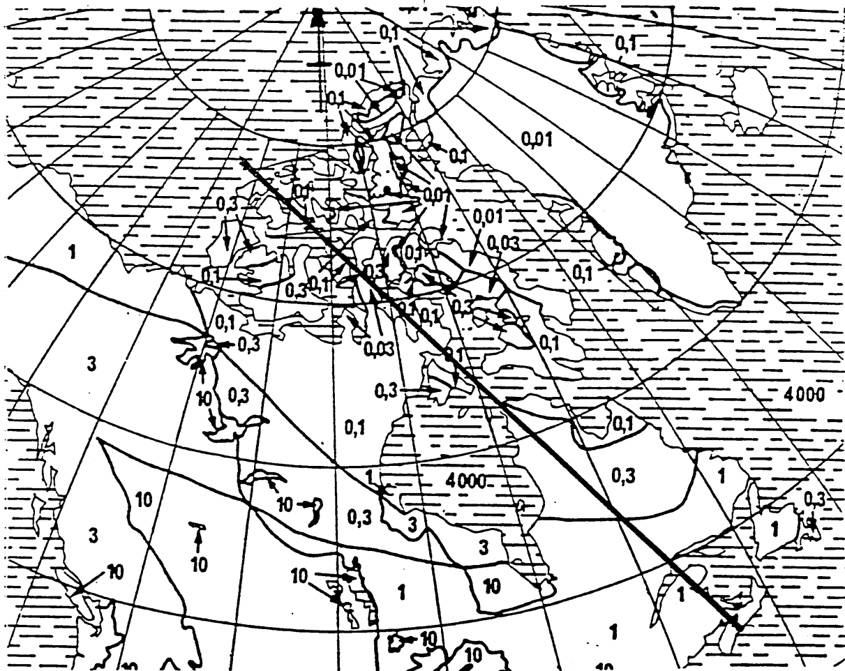
FIGURE 22 VLF ground conductivity map for Canada and the Arctic (mS/m)
