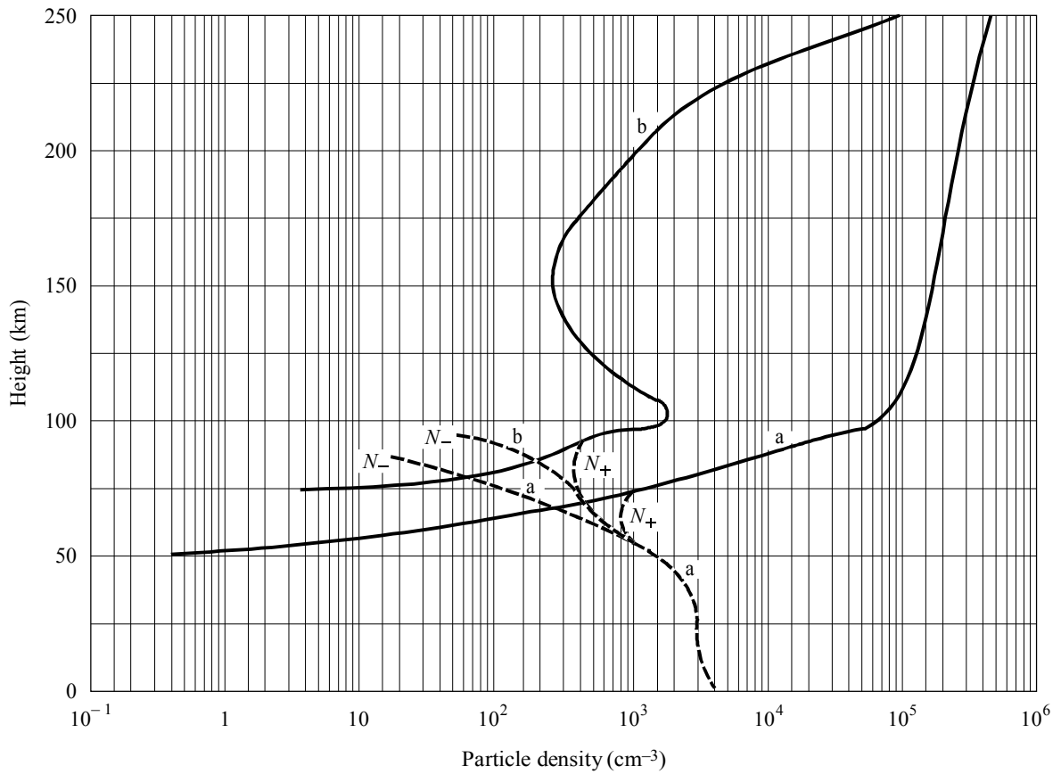
FIGURE 19 Ambient day and night constituent profiles
