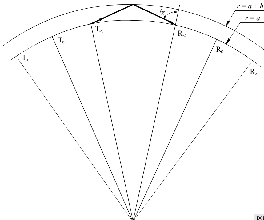
FIGURE 1 Ray path geometry for the wave-hop radio propagation theory (first hop sky wave)
