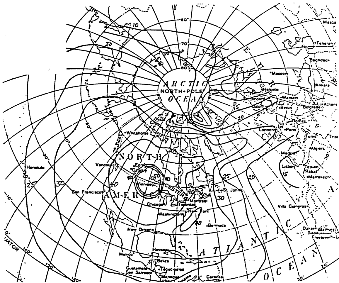
FIGURE 21 Field strength contours ( \text{dB}(\mu\text{V}/\text{m}) ) for 1 kW radiated power, for a hypothetical transmitter located in central Canada. Frequency 24 kHz, for a summer day
