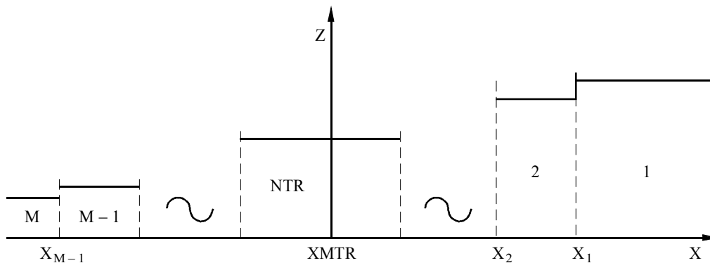
FIGURE 16 Mode conversion model
