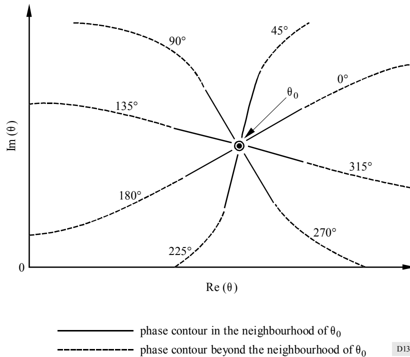
FIGURE 13 Phase contour behaviour near a zero of F(\theta)
