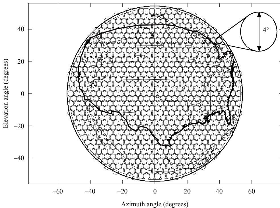
FIGURE 6 USA KUL2 spot beam coverage (Tx and Rx)
