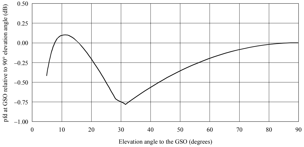
Variation of the pfd received at the GSO computed at 29.75 GHz
