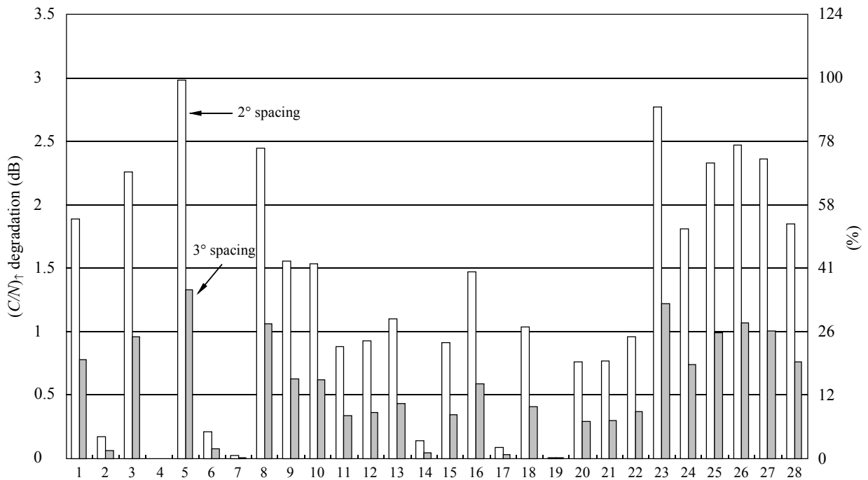
FIGURE 3 Maximum degradation in (C/N)_r of 29.5-30 GHz Recommendation ITU-R S.1328 carriers from single-entry interference at off-axis e.i.r.p. limit level
