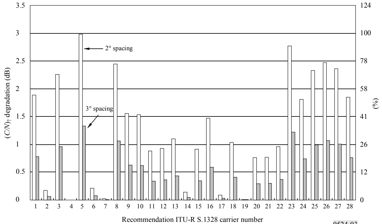
Maximum degradation in (C/N)_T of 29.5-30 GHz Recommendation ITU-R S.1328 carriers from single-entry interference at off-axis e.i.r.p. limit level
