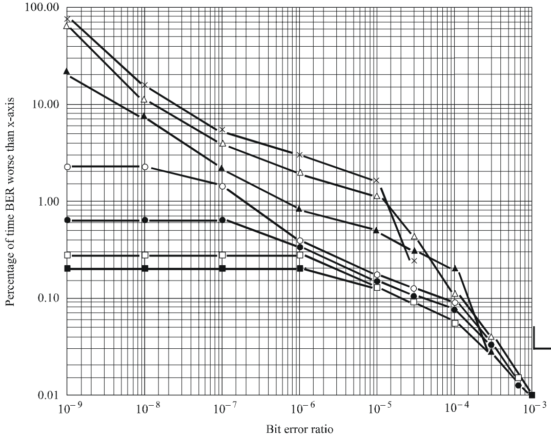
Examination of relationship between the BER measurements and ITU-T Recommendation G.821 parameter measurements
