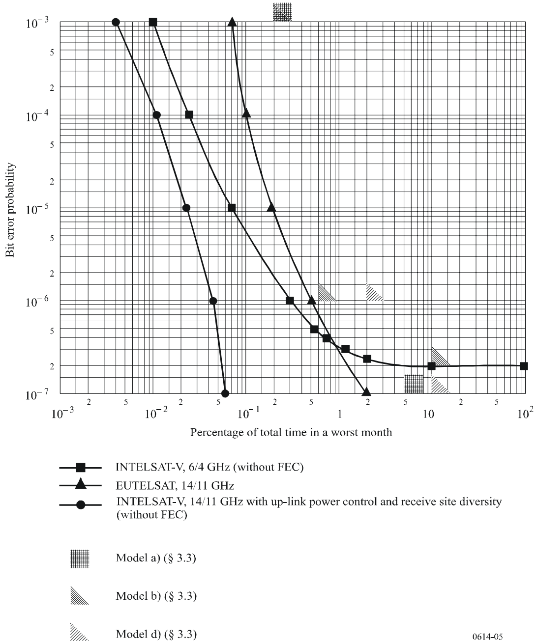
FIGURE 5 Bit error probability versus percentage of total time in a worst month
