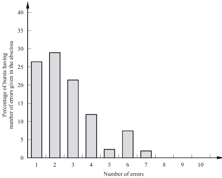
Histogram of number of errors per burst in one 64 kbit/s channel within a multiplex at primary rate of 2 048 kbit/s (ITU-T Recommendation G.704
