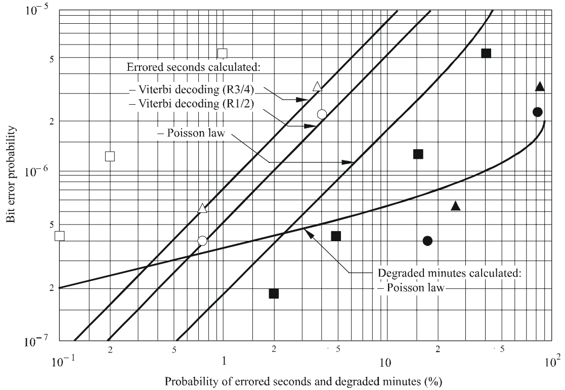
Errored seconds and degraded minutes statistics for a 64 kbit/s bit stream (no data scrambling or differential encoding)
