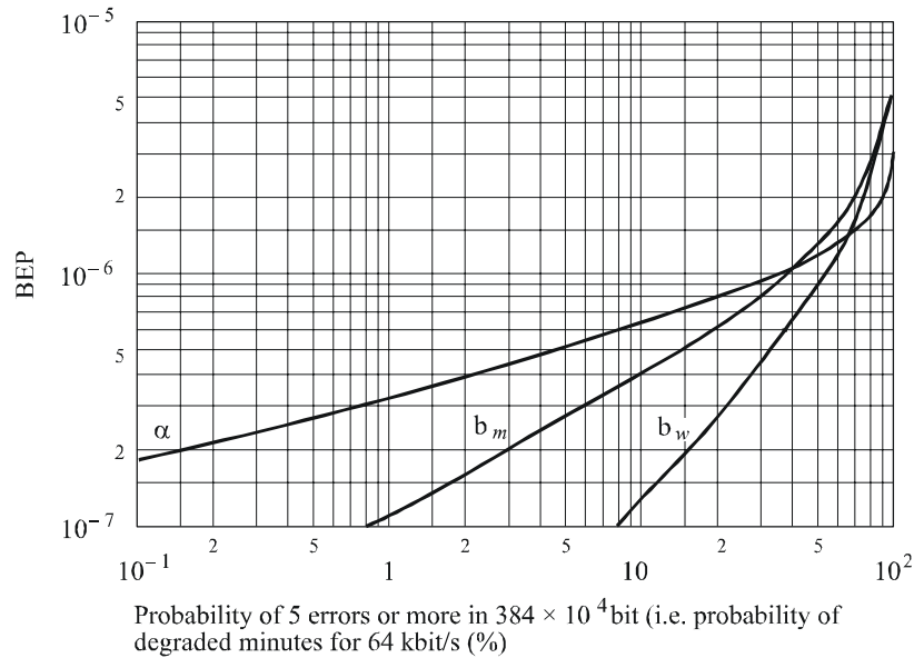
Probability of degraded minutes assuming constant bit error probability
