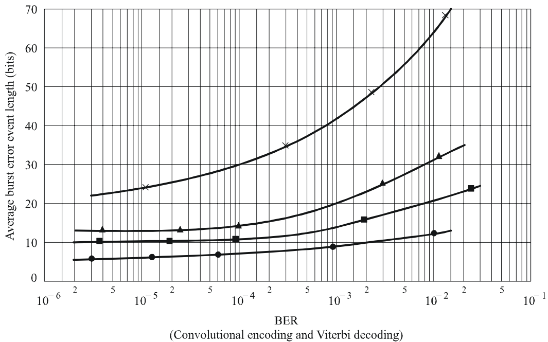
FIGURE 11 Relation between average burst error event length and BER
