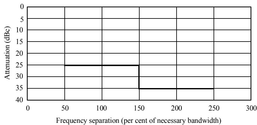
FIGURE 39 OoB mask for aeronautical and maritime mobile
