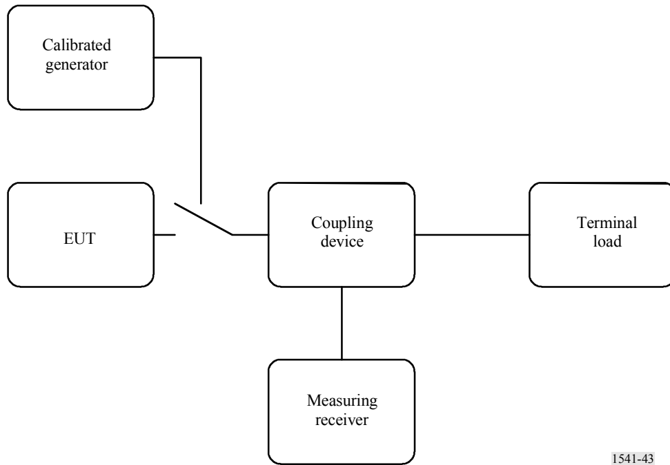
FIGURE 43 Simplified measurement set-up for in-band and OoB emission power to the antenna port
