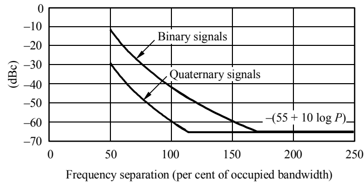
FIGURE 38 Examples of out-of-band masks for aeronautical telemetry (5 Mbit/s at 10 W)
