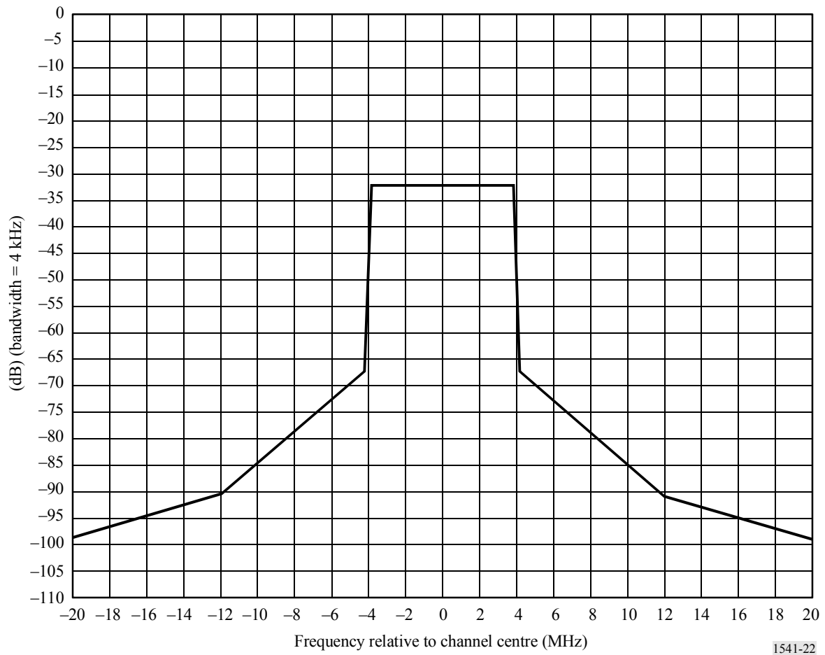
FIGURE 22 Spectrum limit mask for 8 MHz DVB-T (for P = 39 to 50 dBW)
