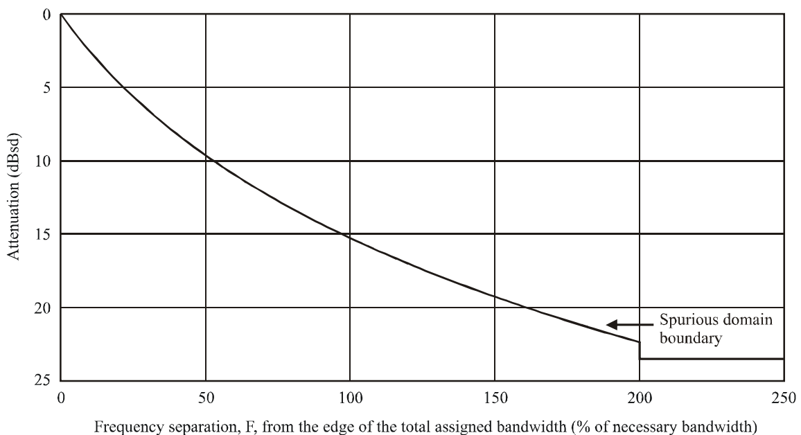
Example application of BSS OoB mask, assuming spurious limit is 23.5 dBsd
