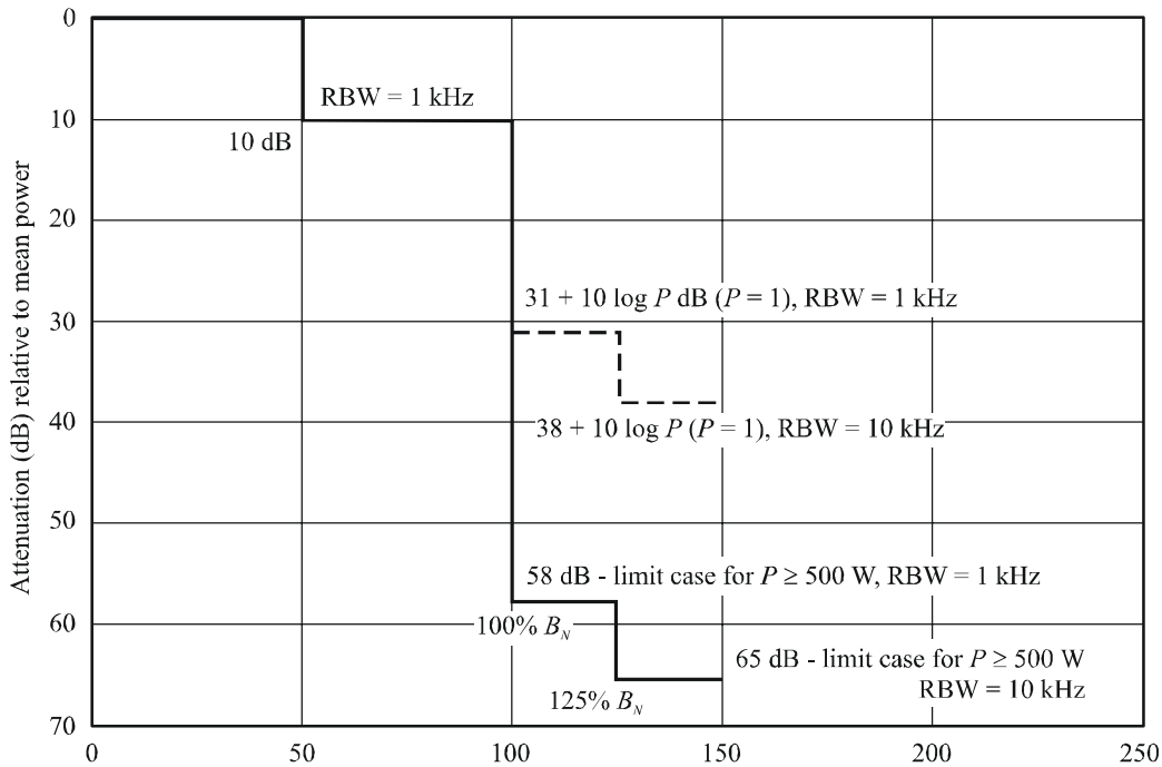
FIGURE 38 Stations operating above 30 MHz in the wideband case of Recommendation ITU-R SM.1539
