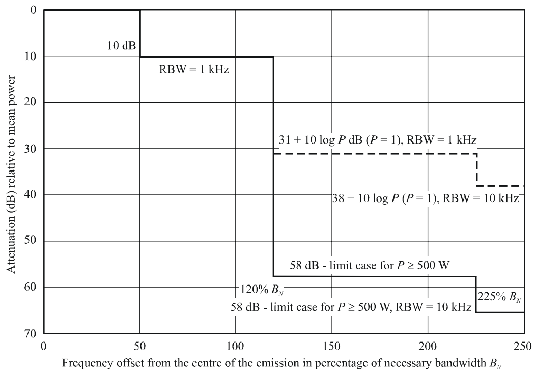
FIGURE 37 Stations operating above 30 MHz in the normal or narrow-band cases of Recommendation ITU-R SM.1539
