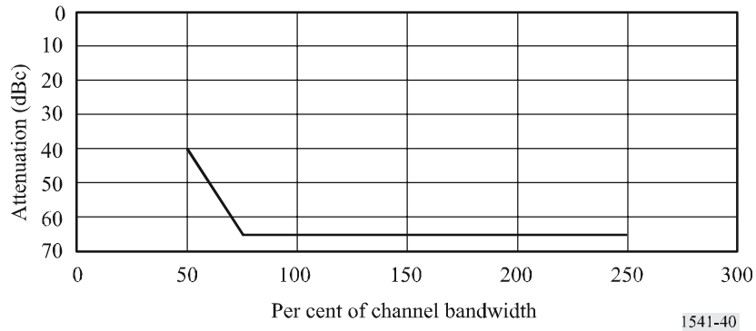
OoB mask for 5 kHz channel bandwidth amplitude companded SSB
