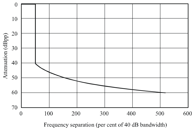
OoB mask for primary radars
