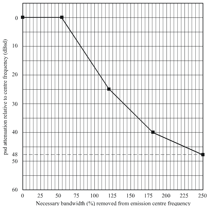
Generic spectrum masks for digital fixed service operating below 30 MHz (see Table 29)
