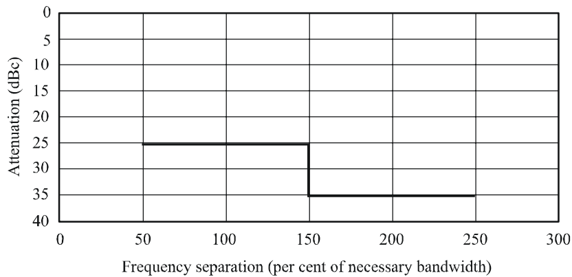
FIGURE 44 OoB mask for aeronautical and maritime mobile
