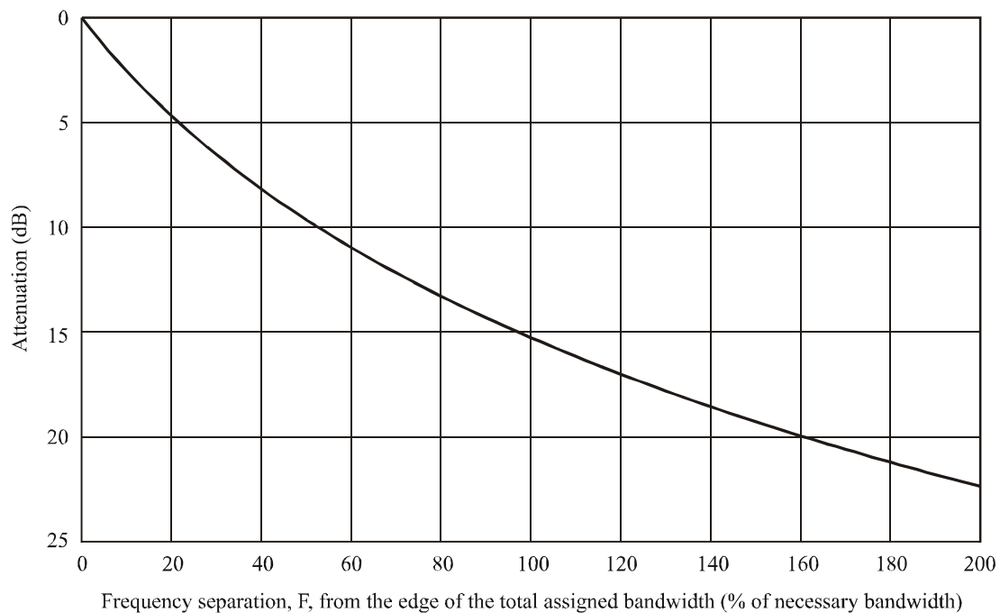
Bss OoB domain emission mask
