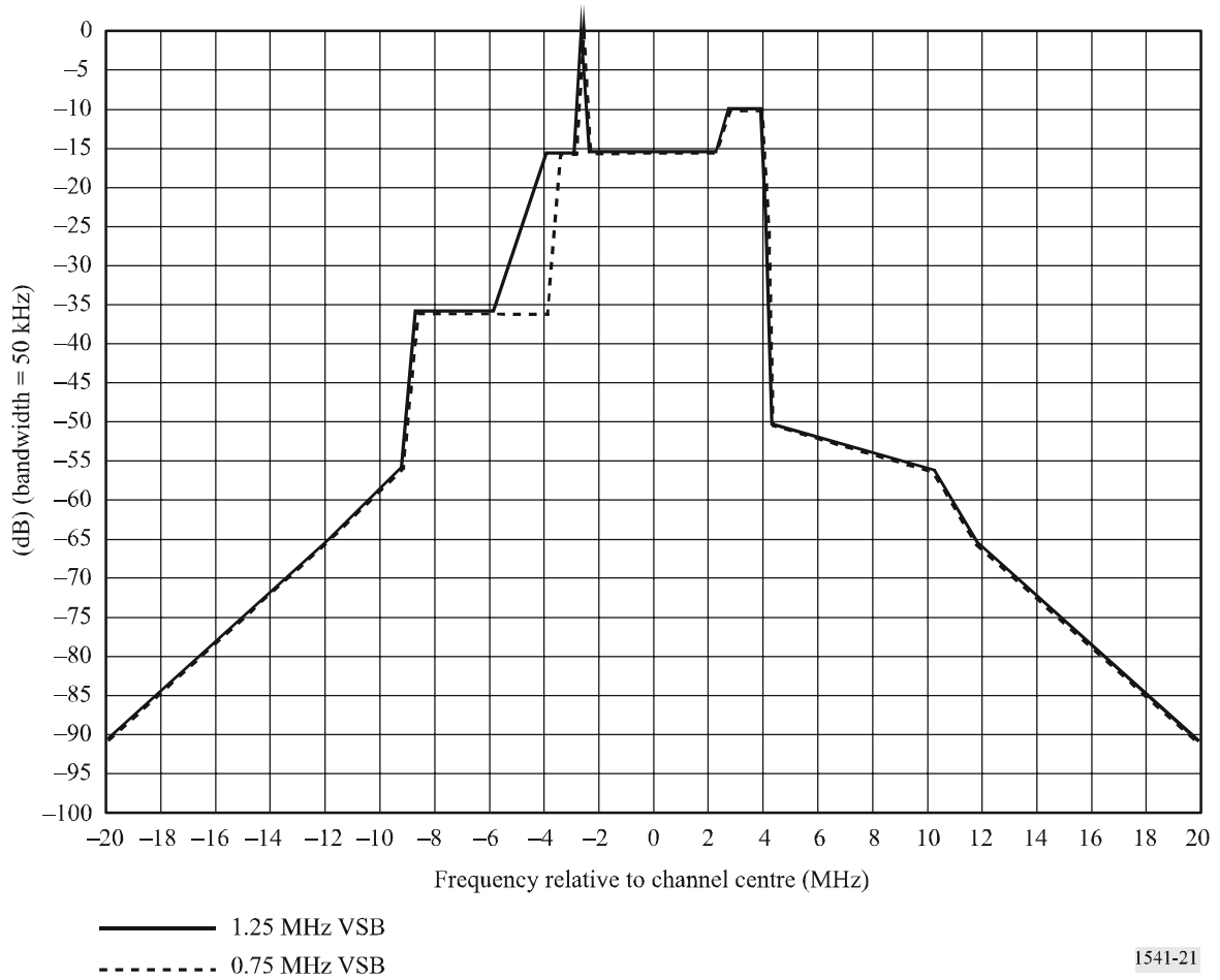
Spectrum limit mask for 8 MHz analogue television, negative modulation (for P = 39 to 50 dBW)
