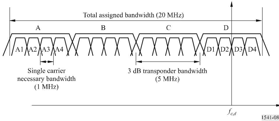
Multicarrier emission with 3 dB transponder bandwidth less than total assigned bandwidth
