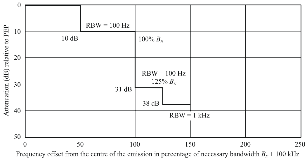
FIGURE 36 Stations operating below 30 MHz in the wideband case of Recommendation ITU-R SM.1539
