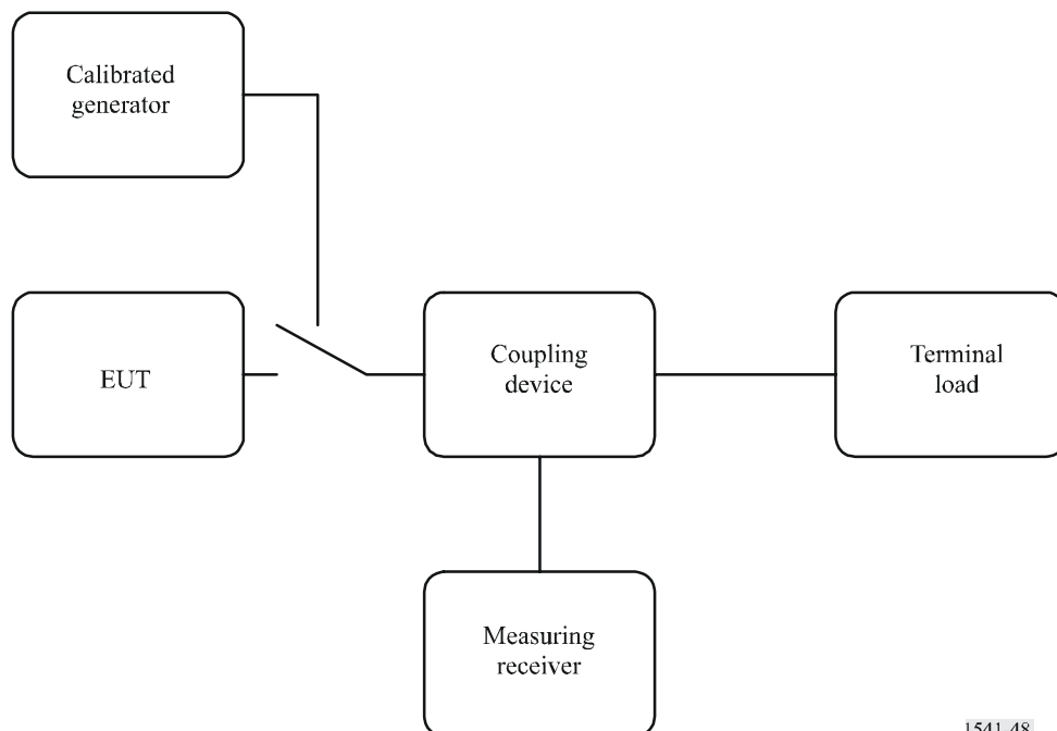
Simplified measurement set-up for in-band and OoB emission power to the antenna port
