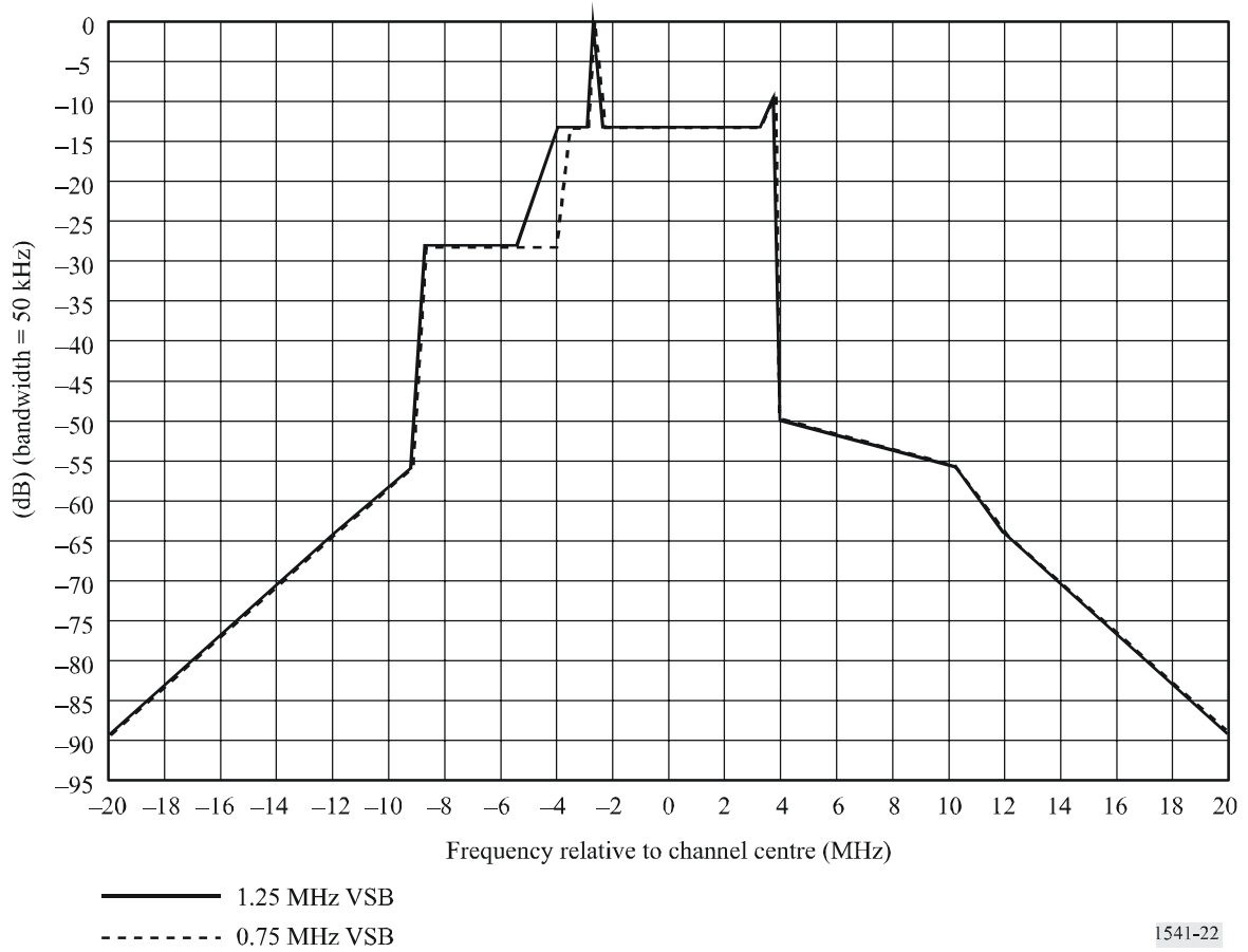
FIGURE 22 Spectrum limit mask for 8 MHz analogue television, positive modulation (for P = 39 to 50 dBW)
