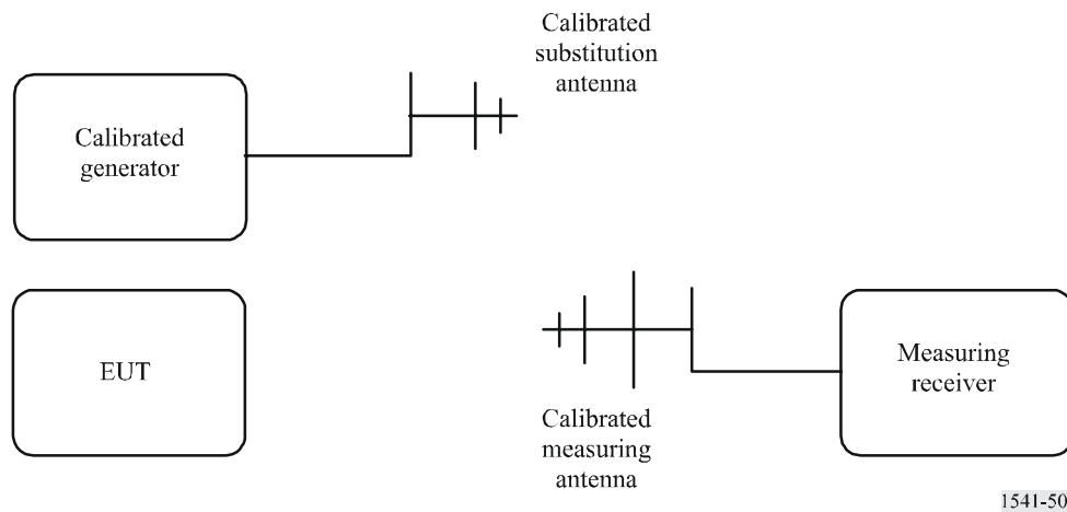
FIGURE 50 Simplified set-up for measuring OoB domain emission e.i.r.p.
