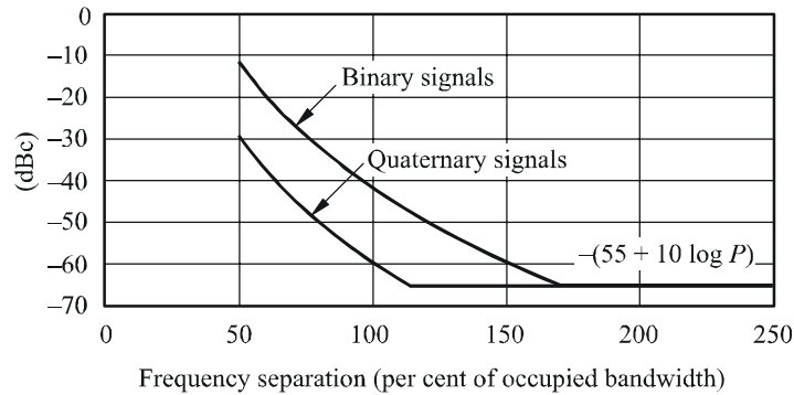
FIGURE 43 Examples of out-of-band masks for aeronautical telemetry (5 Mbit/s at 10 W)
