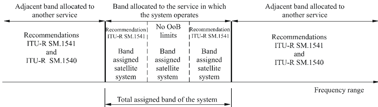
Frequency range where generic OoB masks may apply
