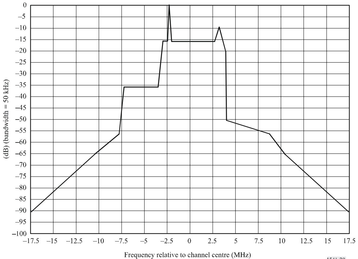
FIGURE 20 Spectrum limit mask for 7 MHz analogue television, negative modulation 0.75 MHz VSB (for P = 39 to 50 dBW)
