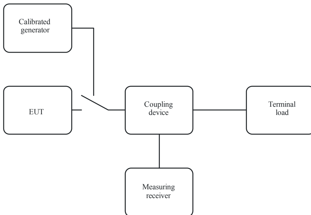
FIGURE 47 Simplified measurement set-up for in-band and OoB emission power to the antenna port
