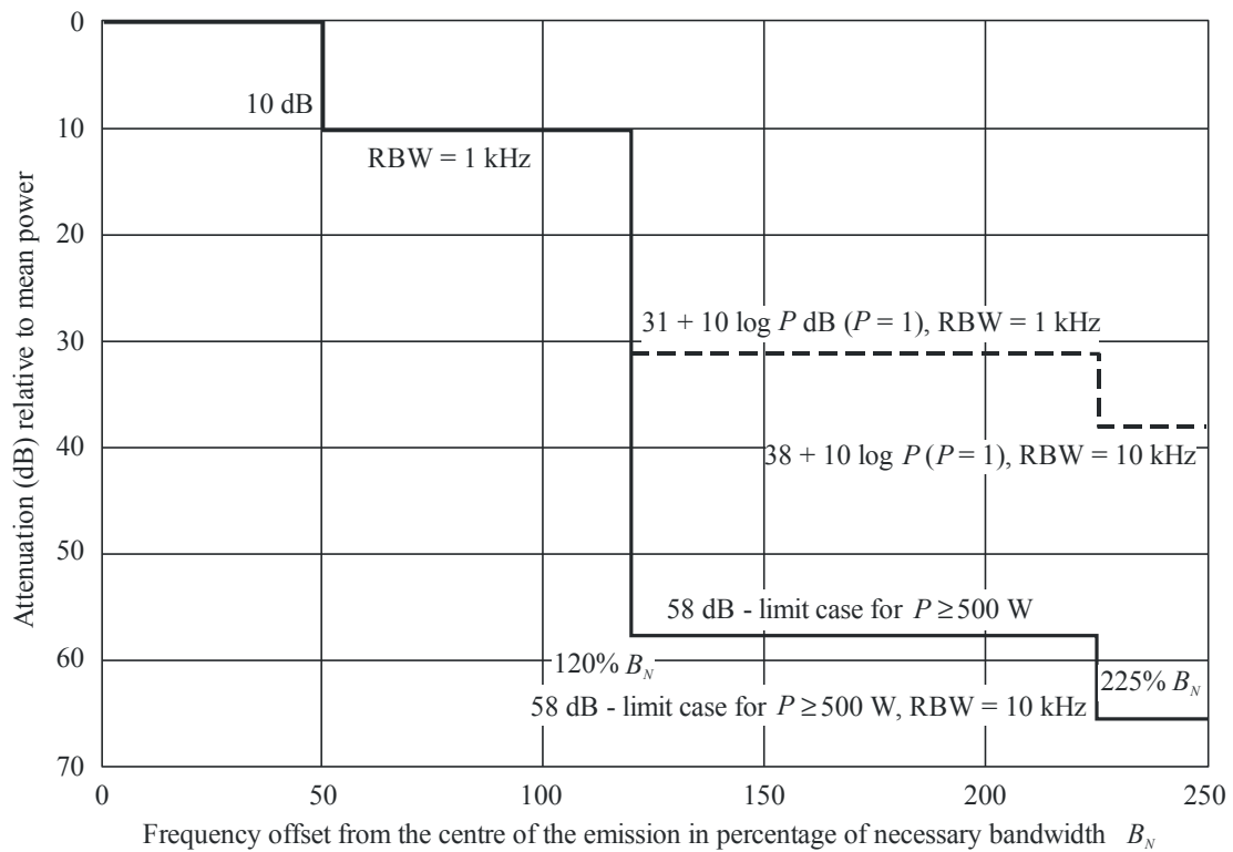
FIGURE 36 Stations operating above 30 MHz in the normal or narrow-band cases of Recommendation ITU-R SM.1539
