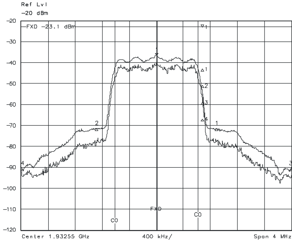
Code division multiple access (IS95) uplink spectrum measured with true mean power measurement function (upper) and trace averaging (lower)
