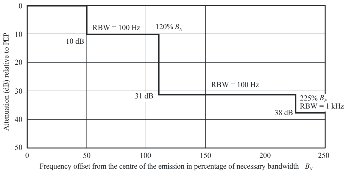
FIGURE 34 Stations operating below 30 MHz in the normal or narrow-band cases of Recommendation ITU-R SM.1539
