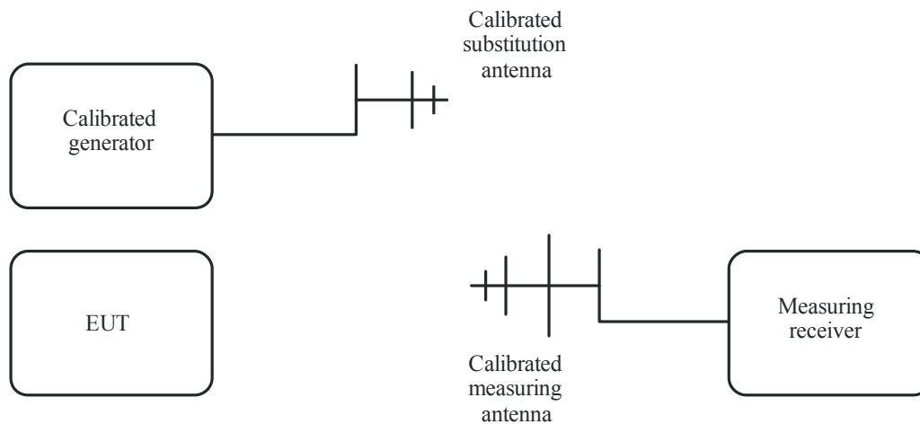
FIGURE 49 Simplified set-up for measuring OoB domain emission e.i.r.p.
