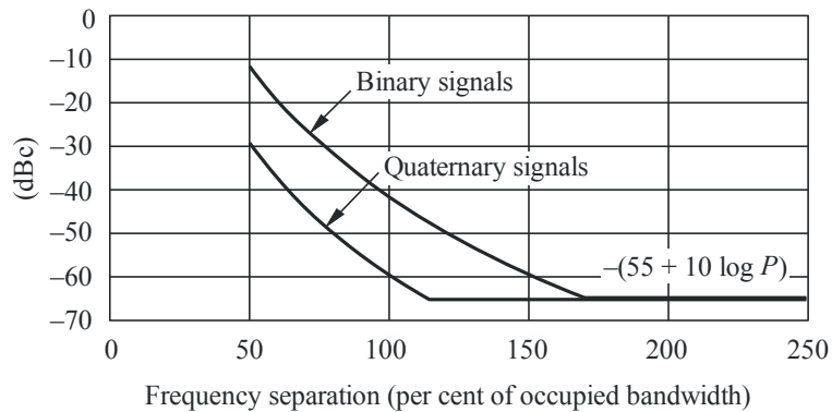
Examples of out-of-band masks for aeronautical telemetry
