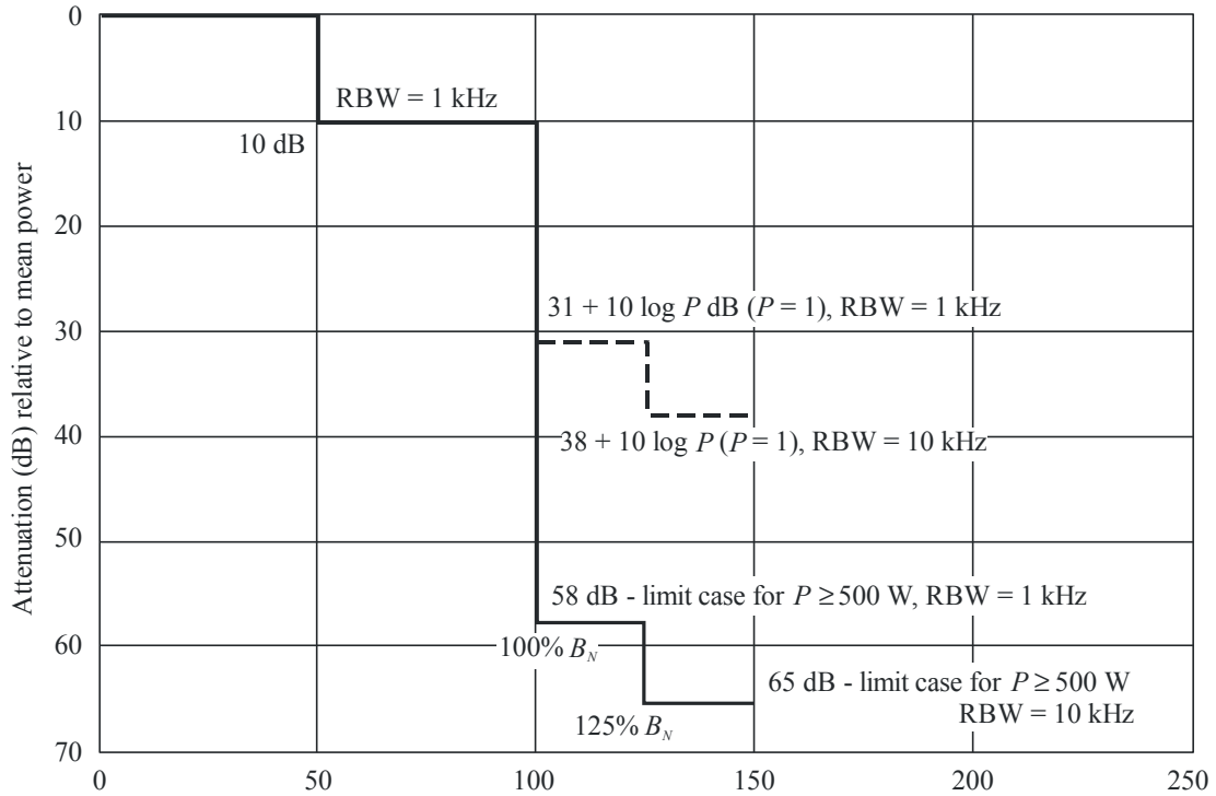
FIGURE 37 Stations operating above 30 MHz in the wideband cases of Recommendation ITU-R SM.1539
