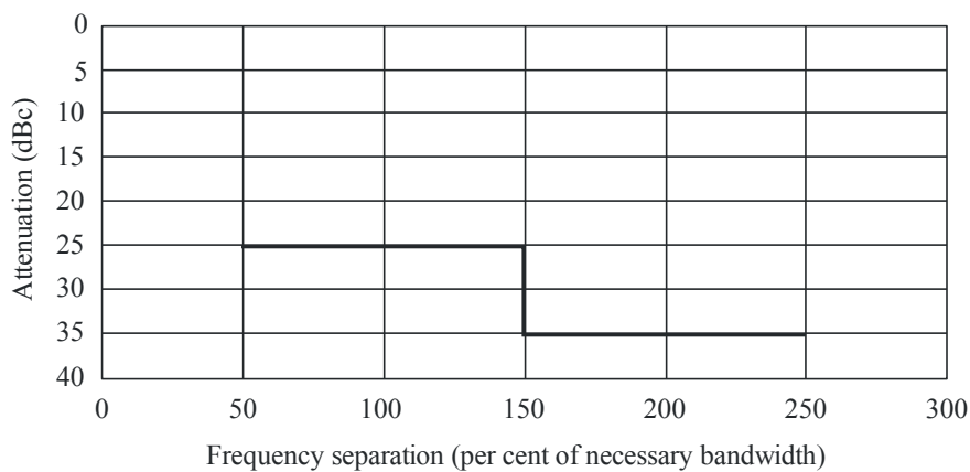
OoB mask for aeronautical and maritime mobile
