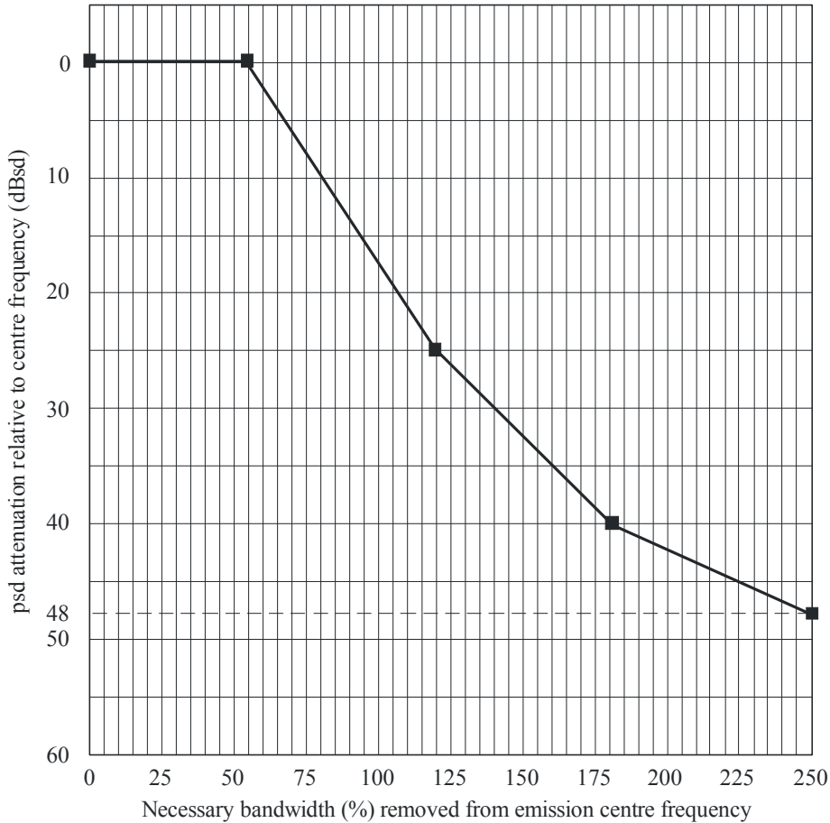
FIGURE 45 Generic spectrum masks for digital fixed service operating below 30 MHz (see Table 29)
