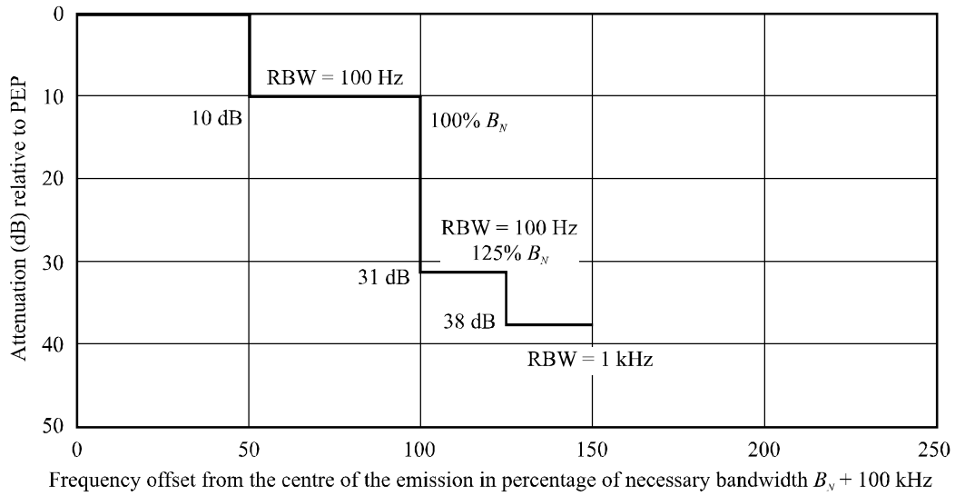
FIGURE 35 Stations operating below 30 MHz in the wideband cases of Recommendation ITU-R SM.1539
