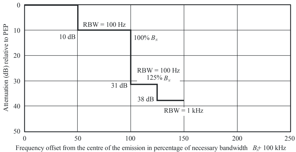
Stations operating below 30 MHz in the wideband cases of Recommendation ITU-R SM.1539
