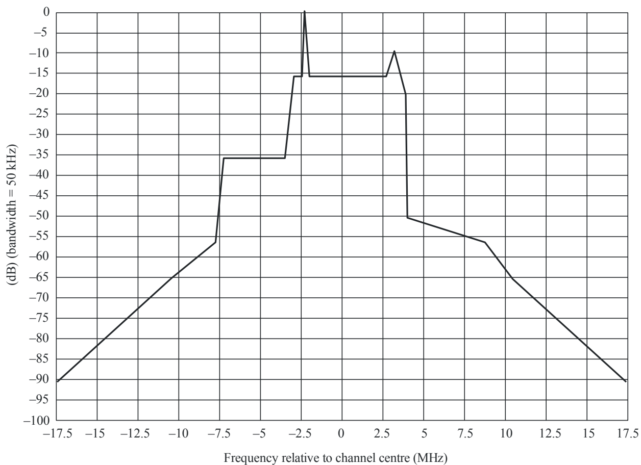
FIGURE 19 Spectrum limit mask for 7 MHz analogue television, negative modulation 0.75 MHz VSB (for P = 39 to 50 dBW)
