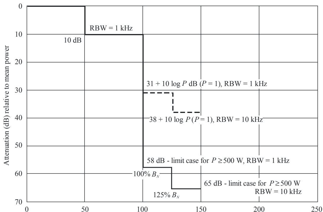
FIGURE 35 Stations operating above 30 MHz in the wideband cases of Recommendation ITU-R SM.1539
