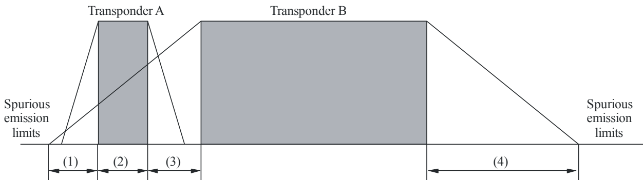
FIGURE 13 Example of applicability of OoB limits to a satellite transponder (this Figure is not drawn to scale)
