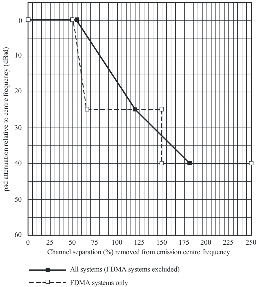
Generic spectrum masks for digital fixed service operating above 30 MHz (see Table 28)
