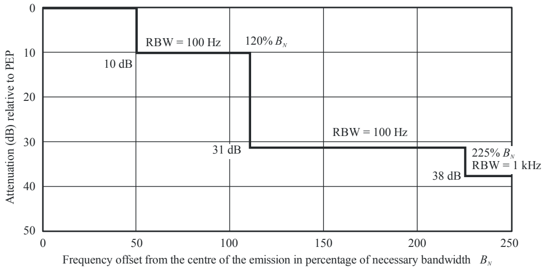
Stations operating below 30 MHz in the normal or narrow-band cases of Recommendation ITU-R SM.1539
