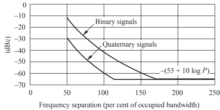
Examples of out-of-band masks for aeronautical telemetry
