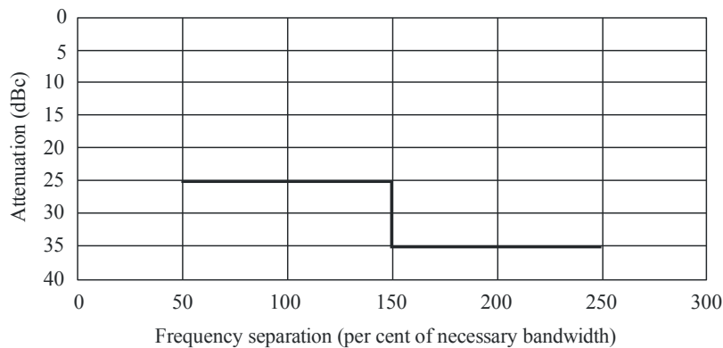
OoB mask for aeronautical and maritime mobile
