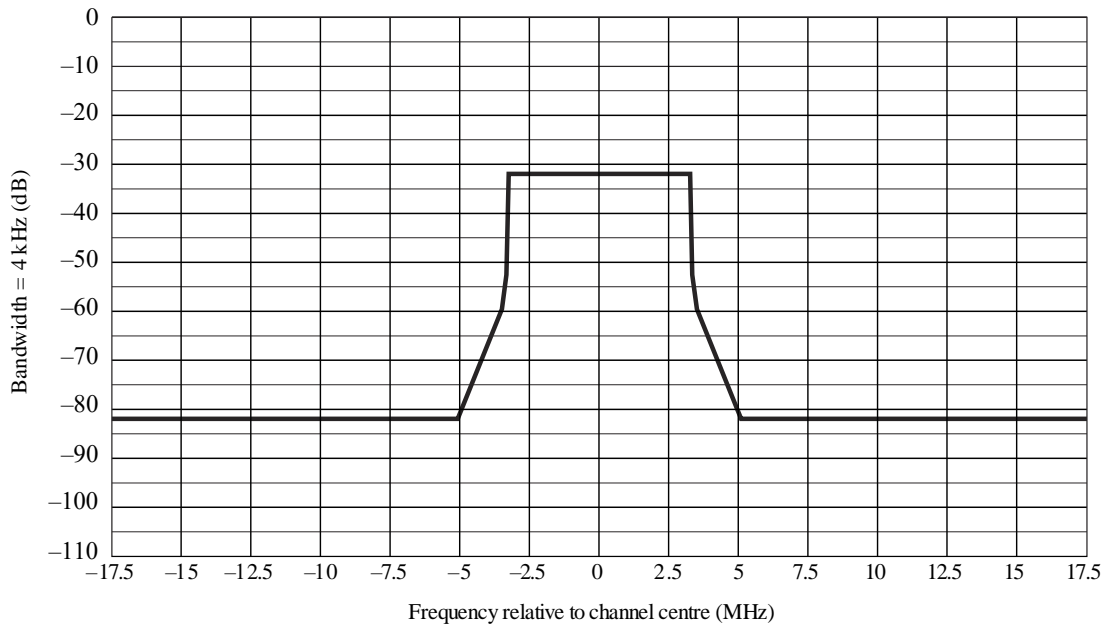
Spectrum limit mask for 7 MHz ISDB-T (for P > 39 dBW)
