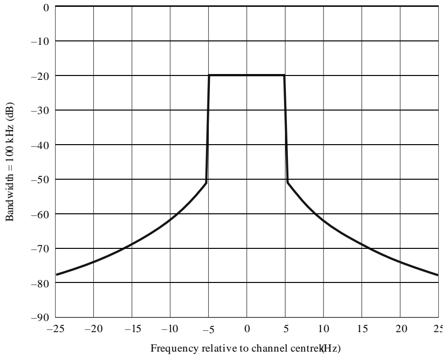
Spectrum limit mask for 10 kHz channelling DRM system
