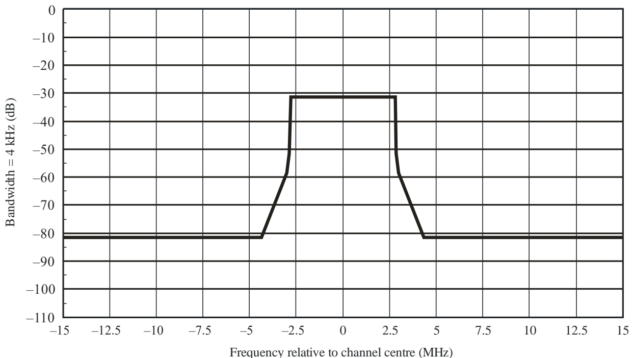
FIGURE 18 Spectrum limit mask for 6 MHz ISDB-T (for P > 39 dBW)
