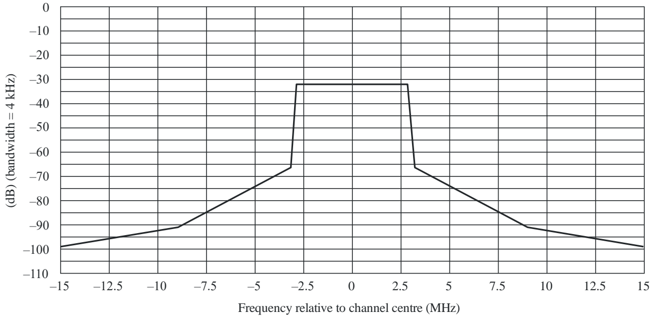
Spectrum limit mask for 6 MHz DVB-T (for P=39 to 50 dBW)
