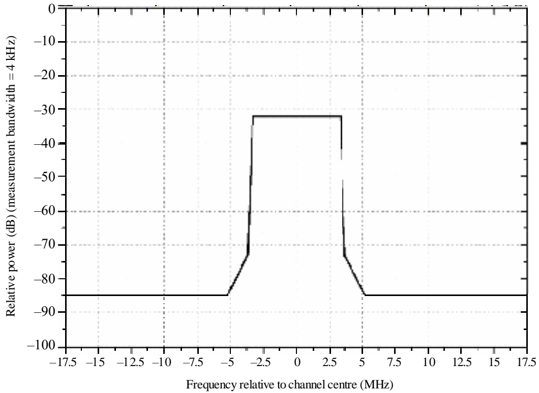
FIGURE 27 Spectrum limit masks for 7 MHz DTMB
