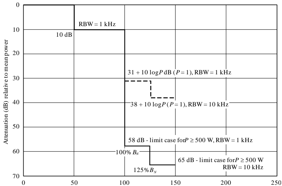
FIGURE 38 Stations operating above 30 MHz in the wideband cases of Recommendation ITU-R SM.1539
