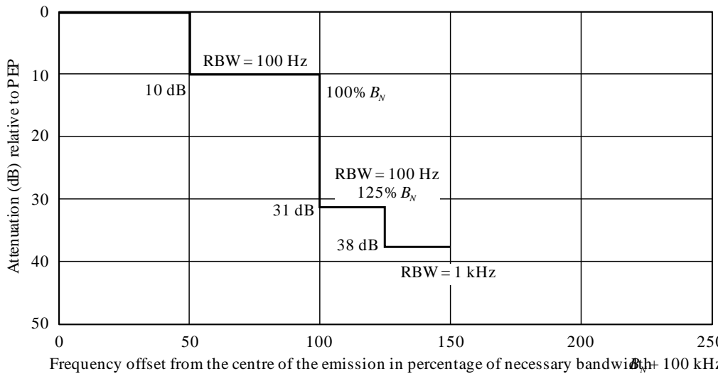
FIGURE 36 Stations operating below 30 MHz in the wideband cases of Recommendation ITU-R SM.1539
