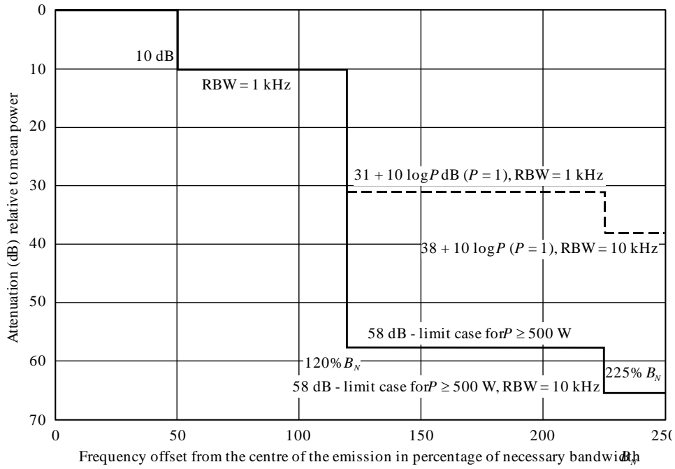
Stations operating above 30 MHz in the normal or narrow-band cases of Recommendation ITU-R SM.1539
