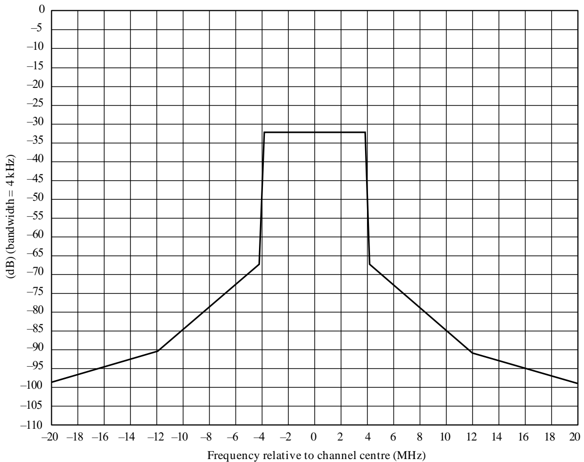
FIGURE 24 Spectrum limit mask for 8 MHz DVB-T (for P = 39 to 50 dBW)
