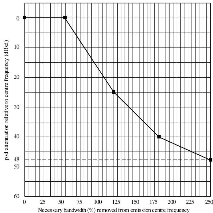
Generic spectrum masks for digital fixed service operating below 30 MHz (see Table 32)
