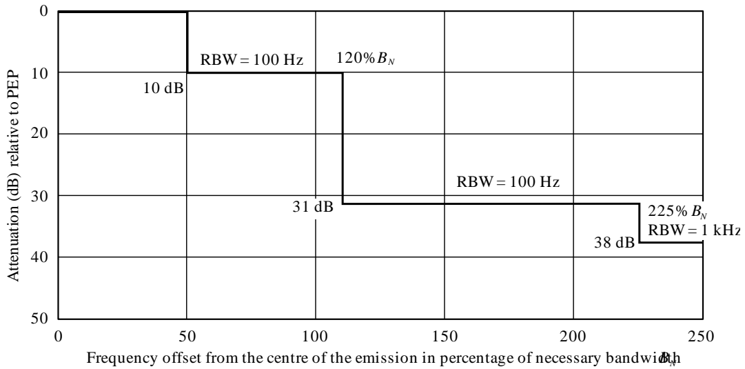
FIGURE 35 Stations operating below 30 MHz in the normal or narrow-band cases of Recommendation ITU-R SM.1539
