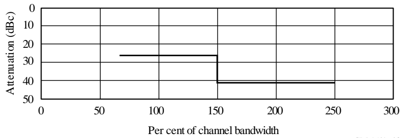
OoB mask for 30 kHz channel bandwidth analogue cellular systems
