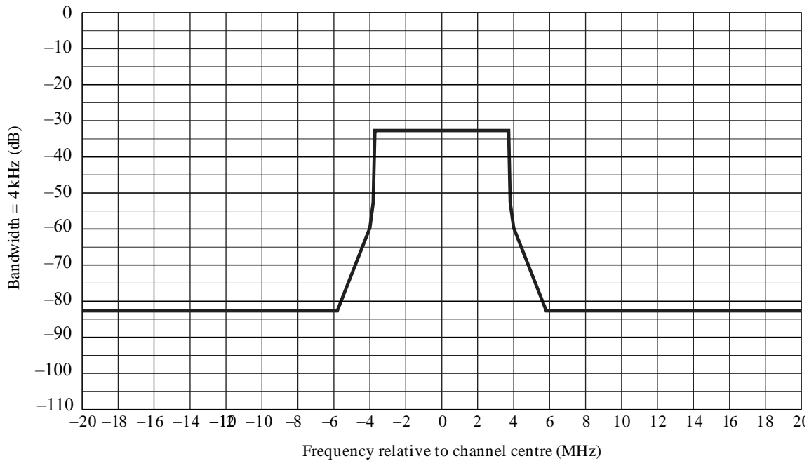
Spectrum limit mask for 8 MHz ISDB-T (for P > 39 dBW)
