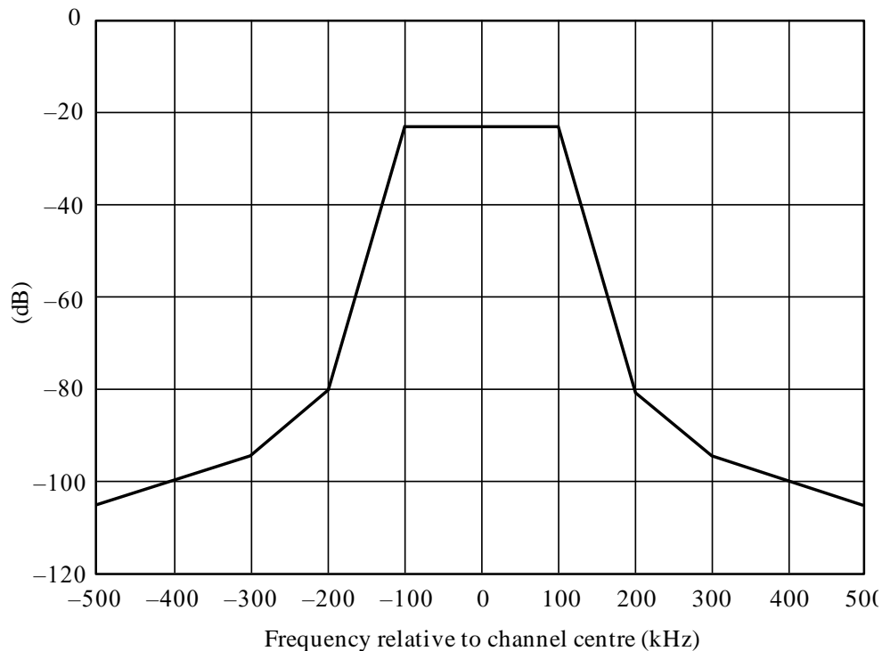
Spectrum limit mask for VHF FM sound broadcasting transmitters (preliminary proposal)
