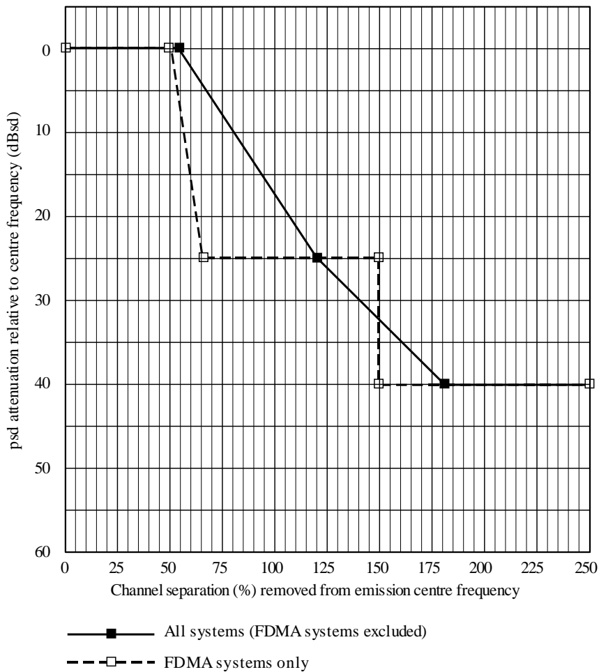
FIGURE 45 Generic spectrum masks for digital fixed service operating above 30 MHz (see Table 31)
