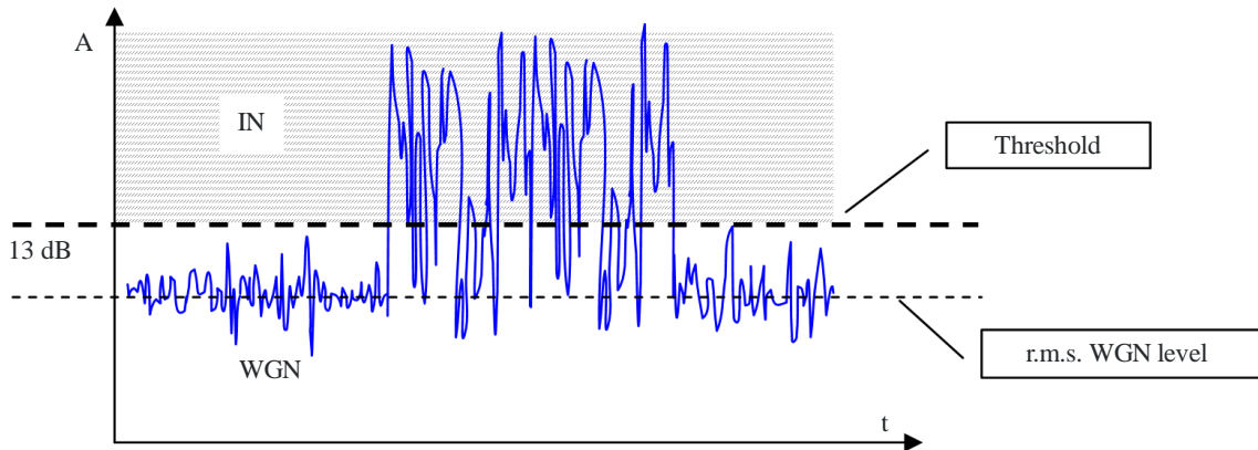
FIGURE 5 Separation of IN and WGN
