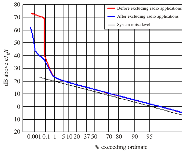
APD graph before and after applying Step 1
