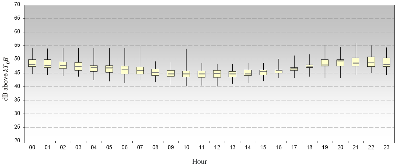
FIGURE 10 r.m.s. WGN results presented as a boxplot Boxplot rural at 5 MHz
