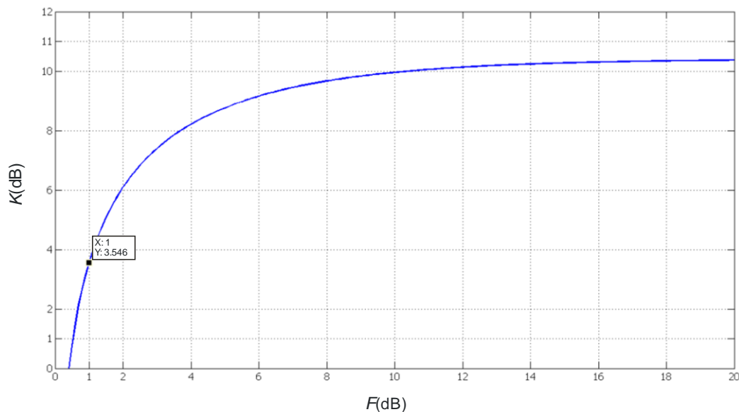
FIGURE 2 Threshold for equipment noise correction
