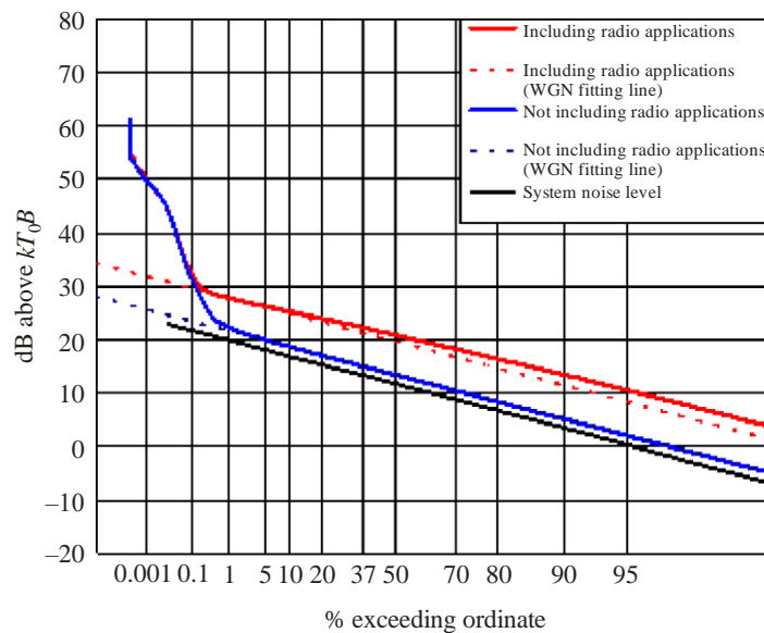
APD graph obtained at two different frequencies
