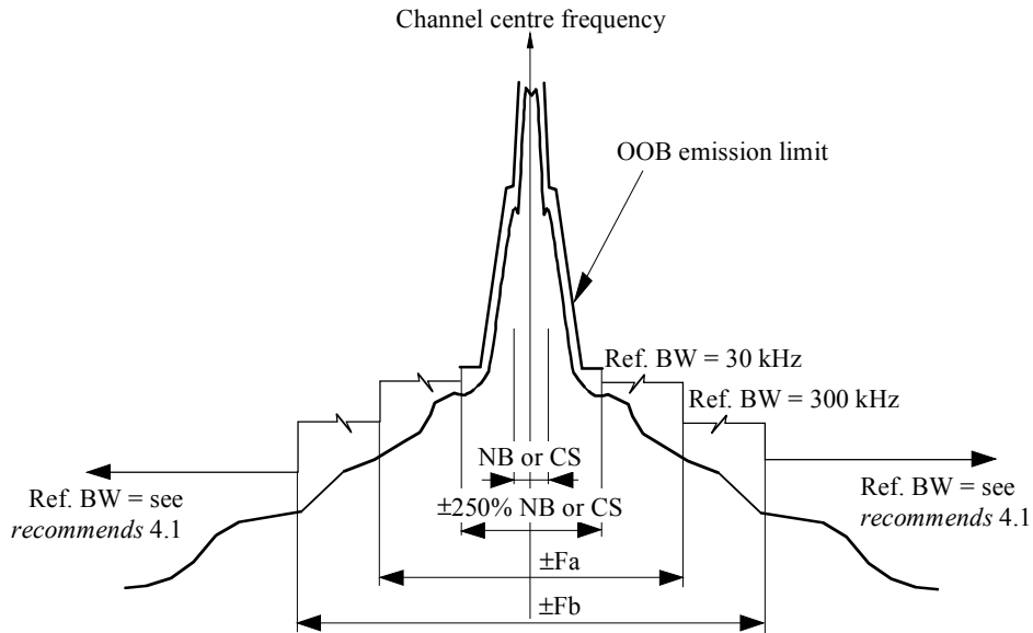
FIGURE 5 Generic Category B land mobile service mask above 1 GHz for unwanted emissions in the spurious domain (refer to Table 13)
