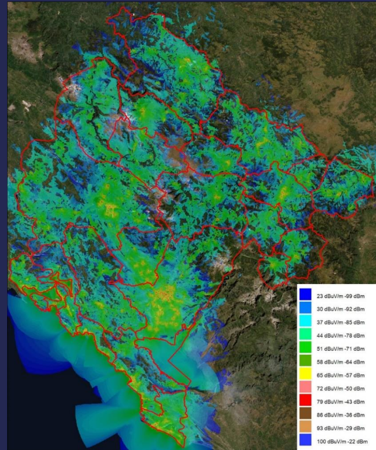
LTE (10 Mbps download) coverage
