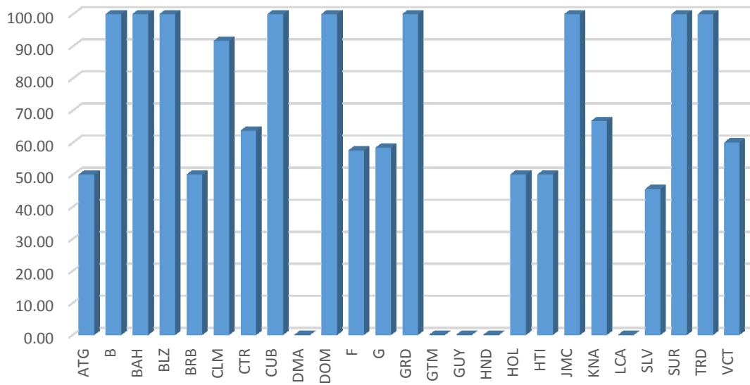
Iteration 19- Percentage of assignable channels (1.25dB margin)
