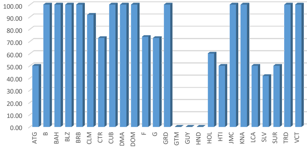
Iteration 23- Percentage of assignable channels (1.25dB margin), ignoring self-interference and interference to the wanted requirement
