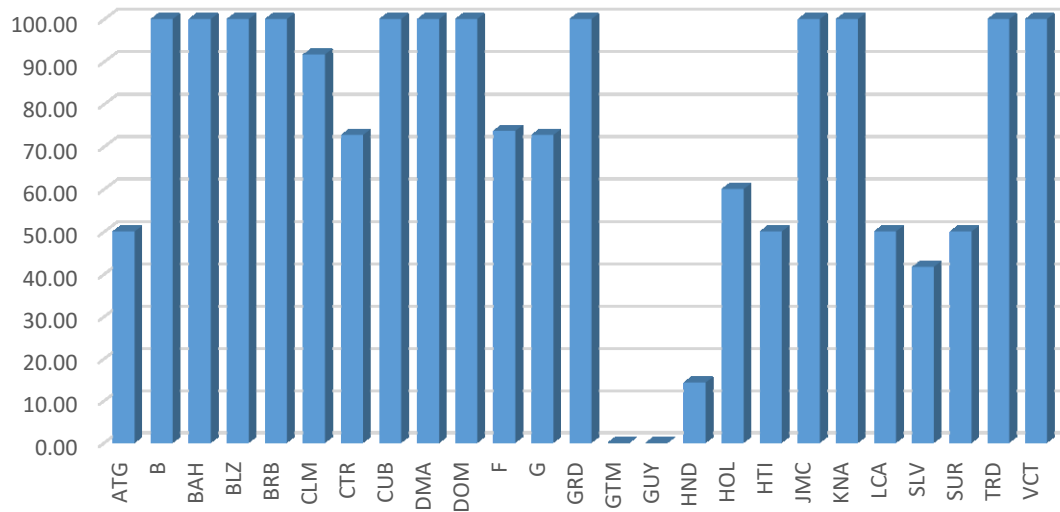
Iteration 24- Percentage of assignable channels (1.25dB margin), ignoring self-interference and interference to the wanted requirement
