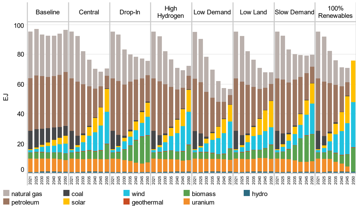
Figure 9 Primary Energy
