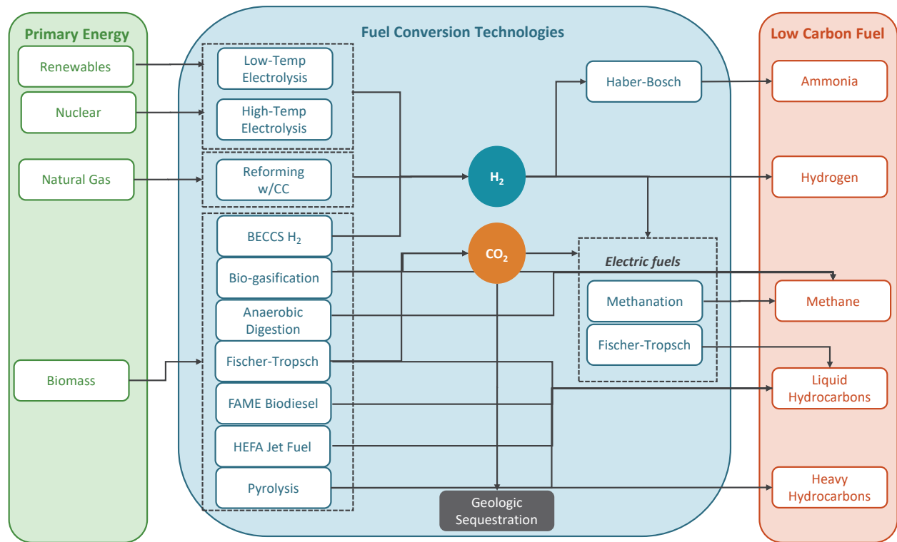
Figure 4 Low-Carbon Fuel Production Pathways
