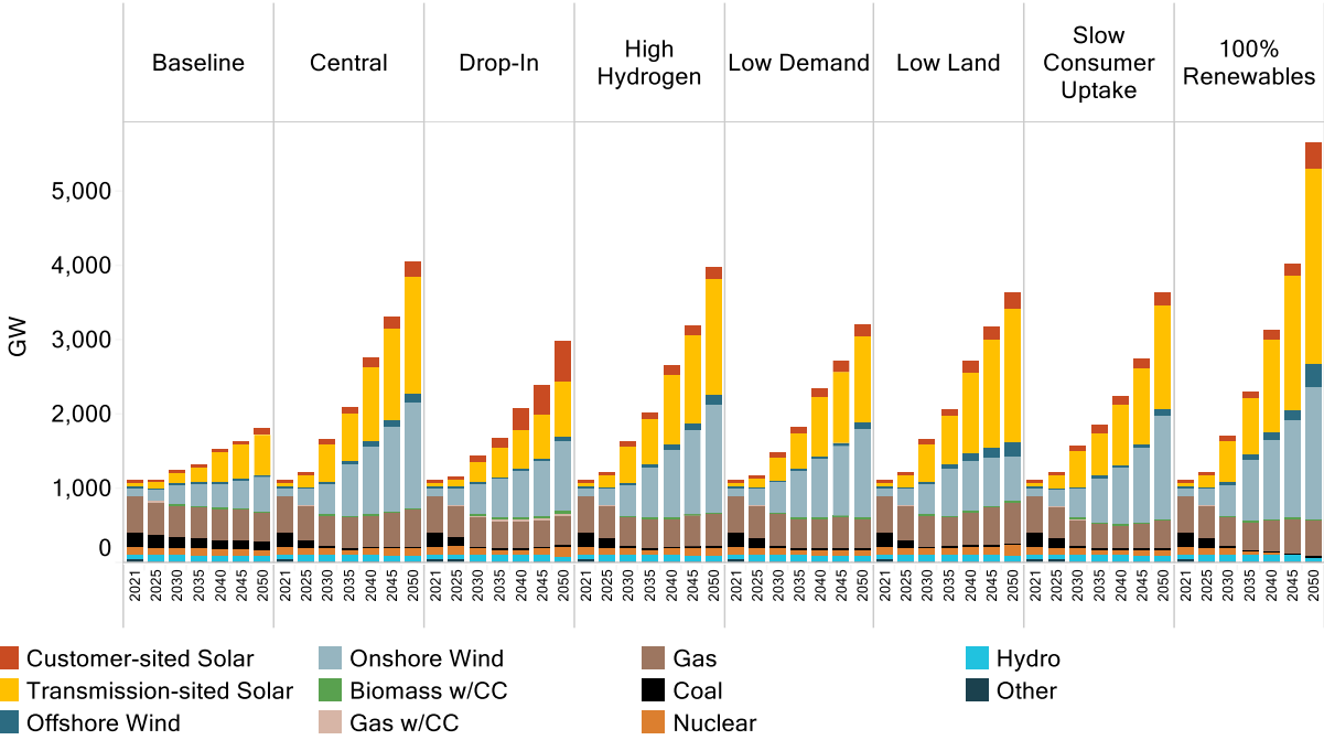
Figure 20 Electricity Generation Capacity
