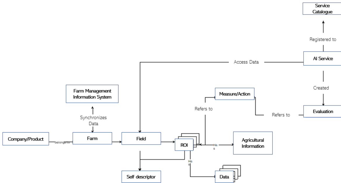
Figure 2: Data flow and access optimization for digital agriculture
