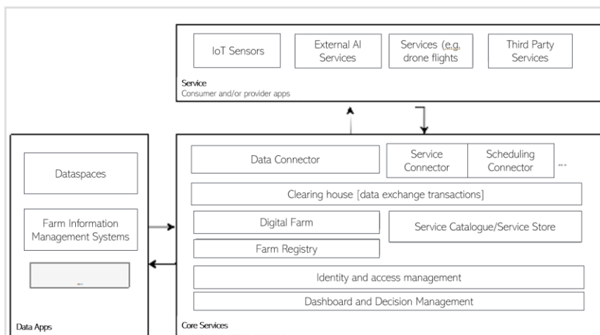
Figure 3: Overview of Technical System Architecture
