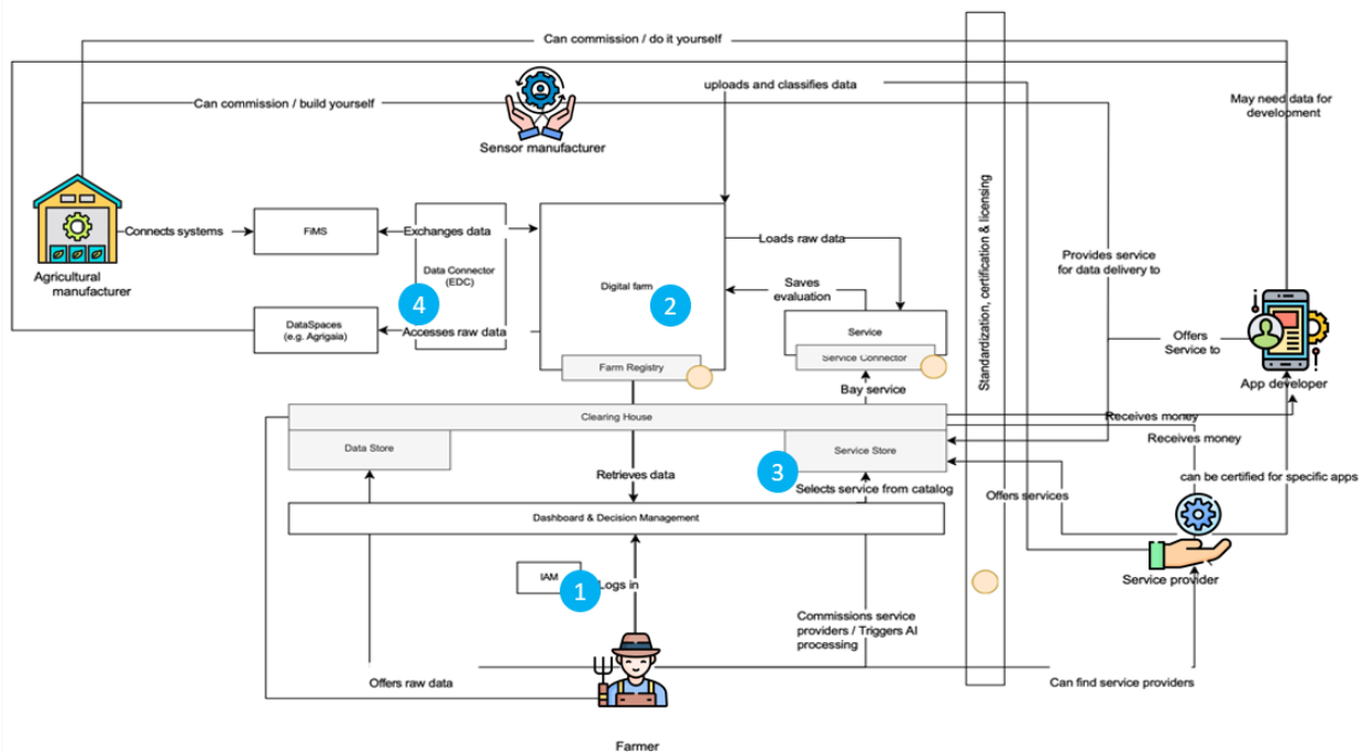
Figure 1: Facilitating data exchanges between stakeholders [b-NALAMKI]
