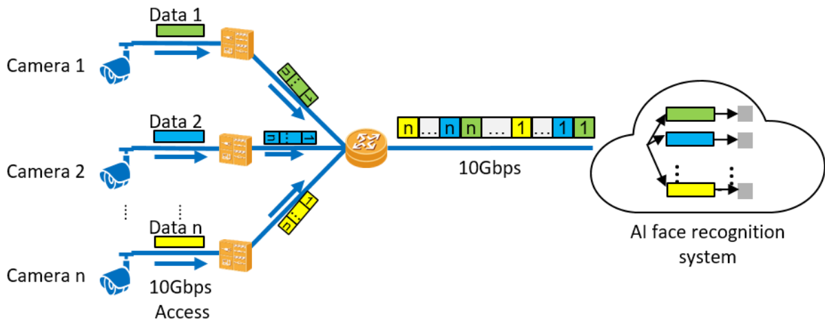
Figure 2 Metro gate control face recognition system architecture.
