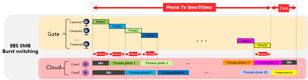
Figure 4 Application-aware data forwarding.
